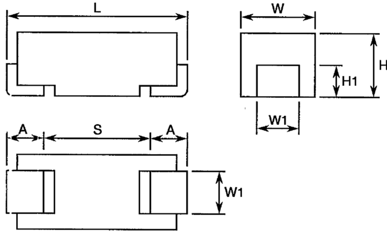
FIGURE 2 - PHYSICAL DIMENSIONS
