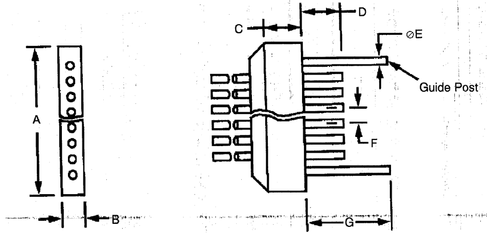
FIGURE 2.1(b) - CONNECTORS RECEPTACLE - FEMALE CONTACT
