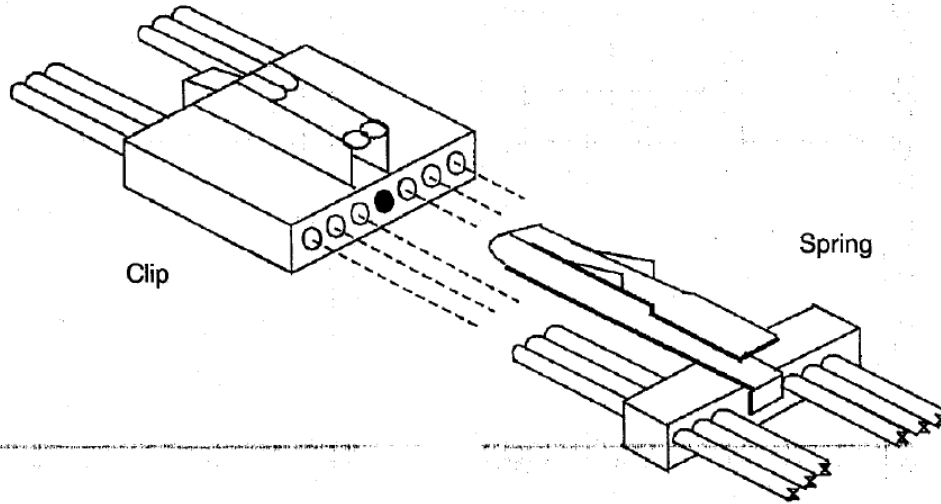
FIGURE 2.4 – LATCHING
