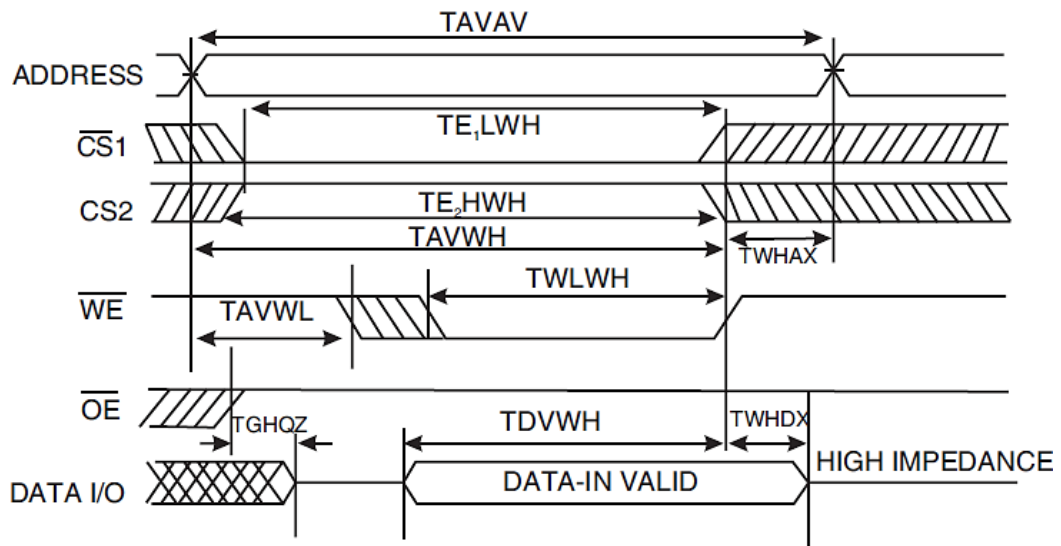
WRITE CYCLE 1: \overline{WE} CONTROLLED, \overline{OE} HIGH DURING WRITE (NOTE 1)
