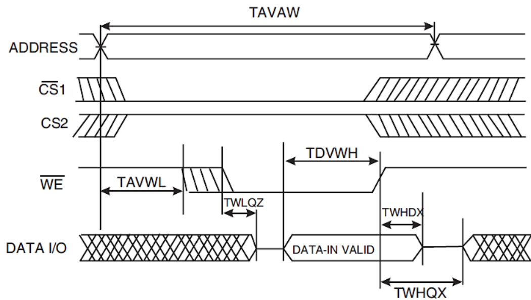
WRITE CYCLE 2: \overline{WE} CONTROLLED, \overline{OE} LOW (NOTE 1)
