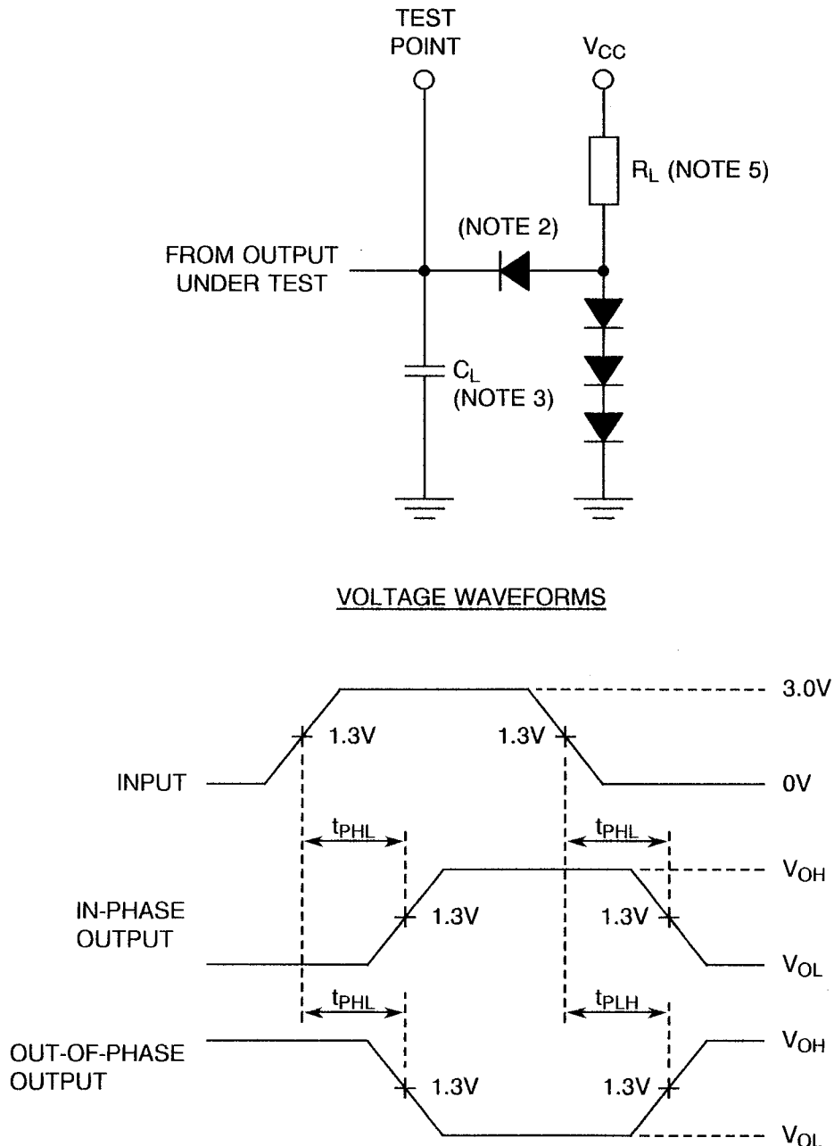
FIGURE 4(h) - DYNAMIC TEST AND SWITCHING WAVEFORMS
