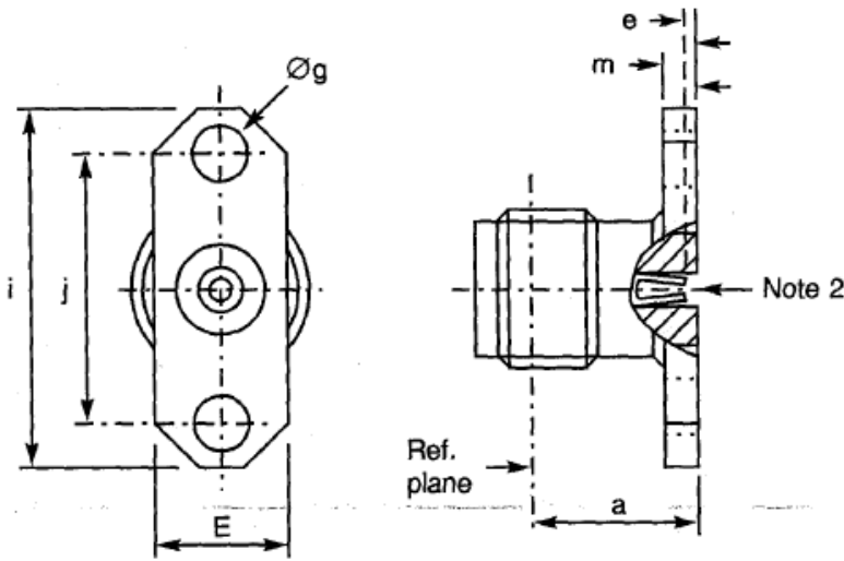
FIGURE 2(b) - VARIANTS (CONTINUED) VARIANT 80 – 2-HOLE FLANGE RECEPTACLE
