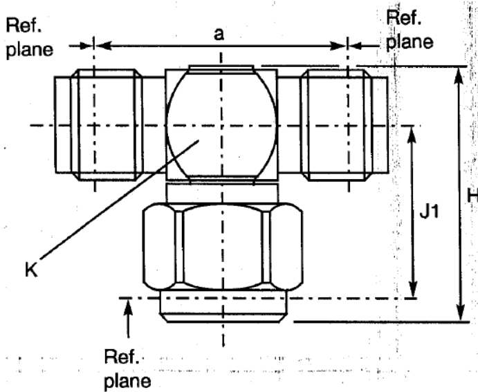
FIGURE 2(b) – VARIANTS (CONTINUED) VARIANT 06 – T-ADAPTOR, FEMALE – FEMALE/MALE
