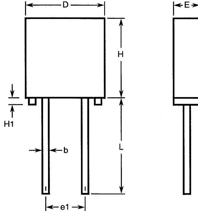
FIGURE 2 - PHYSICAL DIMENSIONS
