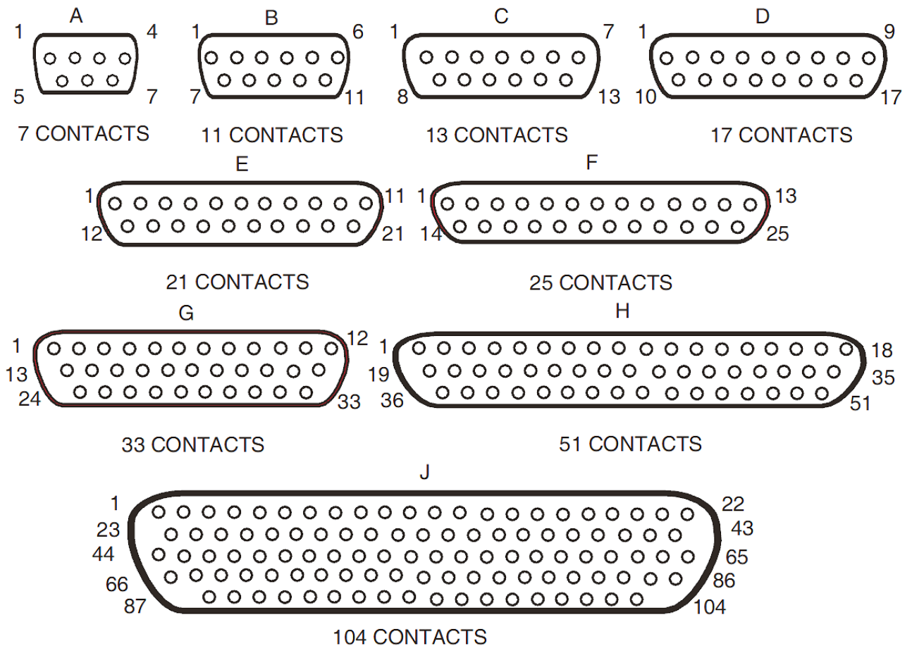
FIGURE 2(b) - CONTACT ARRANGEMENTS
