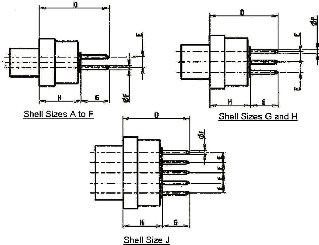
FIGURE 2(c) - REAR END
