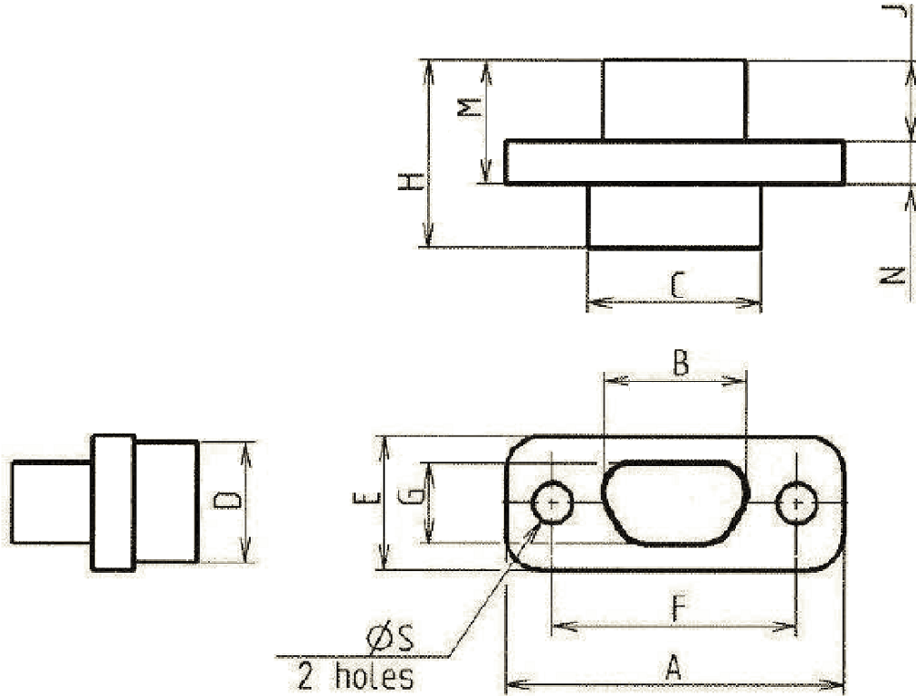
FIGURE 2(a) - CONNECTOR SHELL
