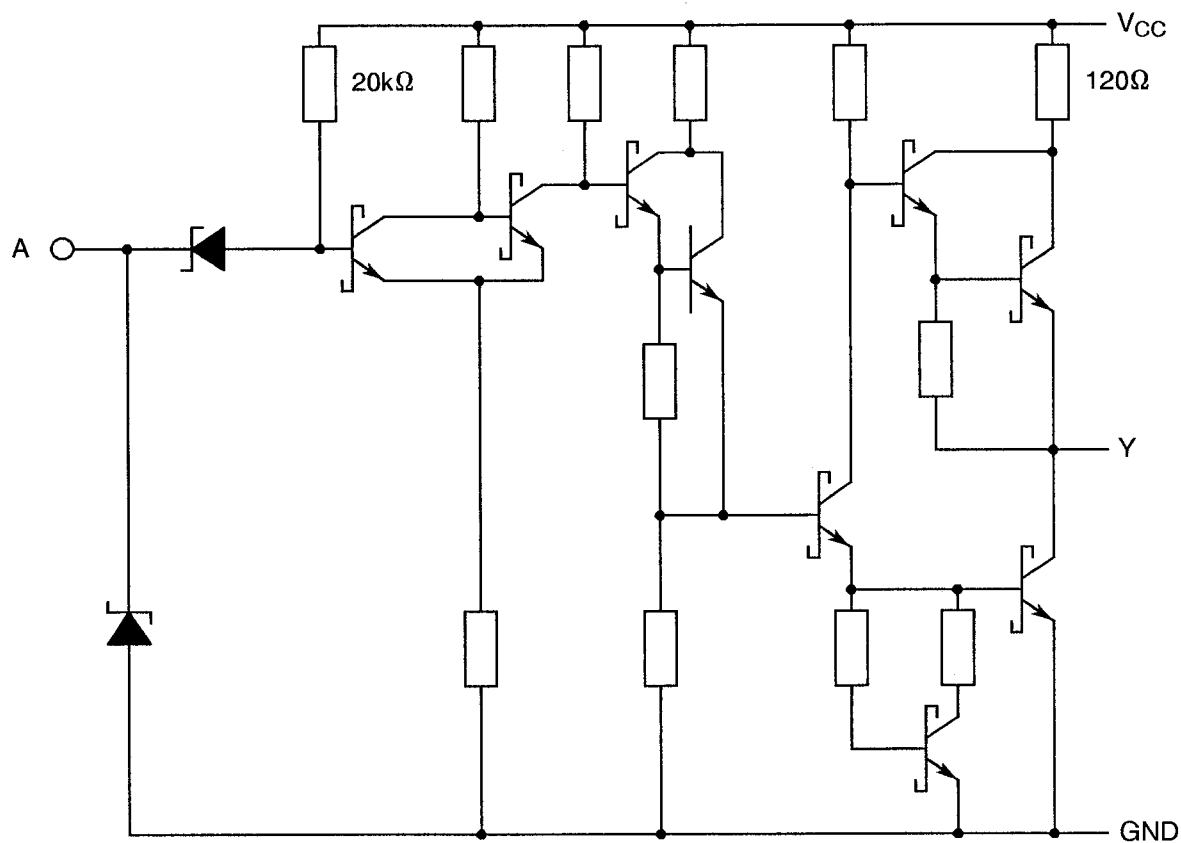
FIGURE 3(c) - CIRCUIT SCHEMATIC (EACH INVERTER)
