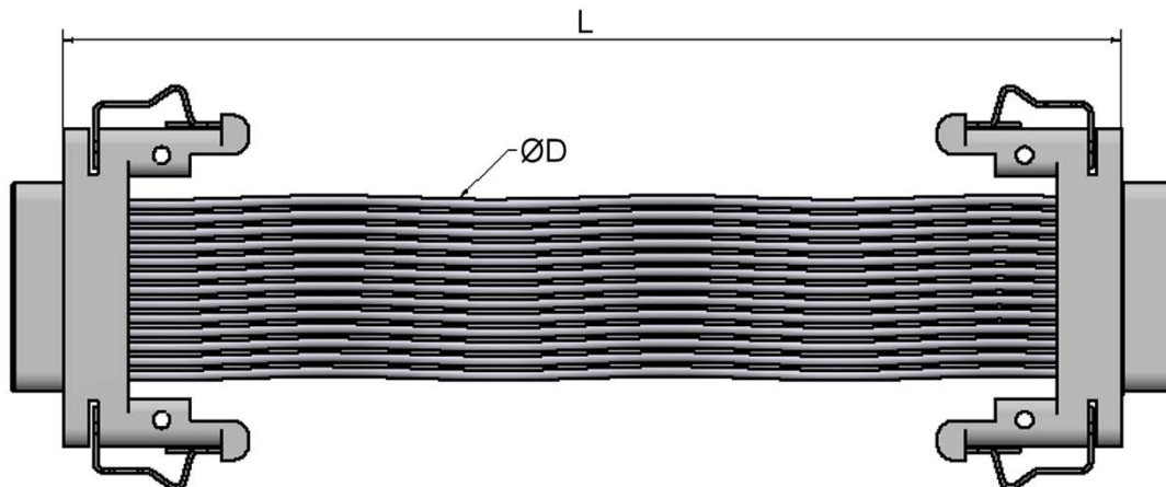
FIGURE 2.1N – VARIANT 08 – JUMPER, CONNECTORS 1 AND 2: VARIANT 01
