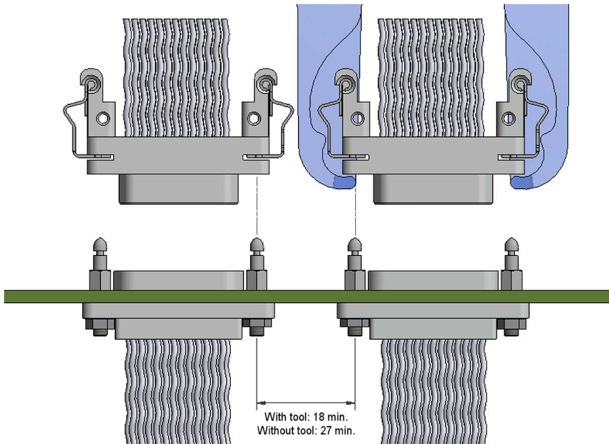
FIGURE 2.3.1 – HORIZONTAL MINIMUM SPACING
