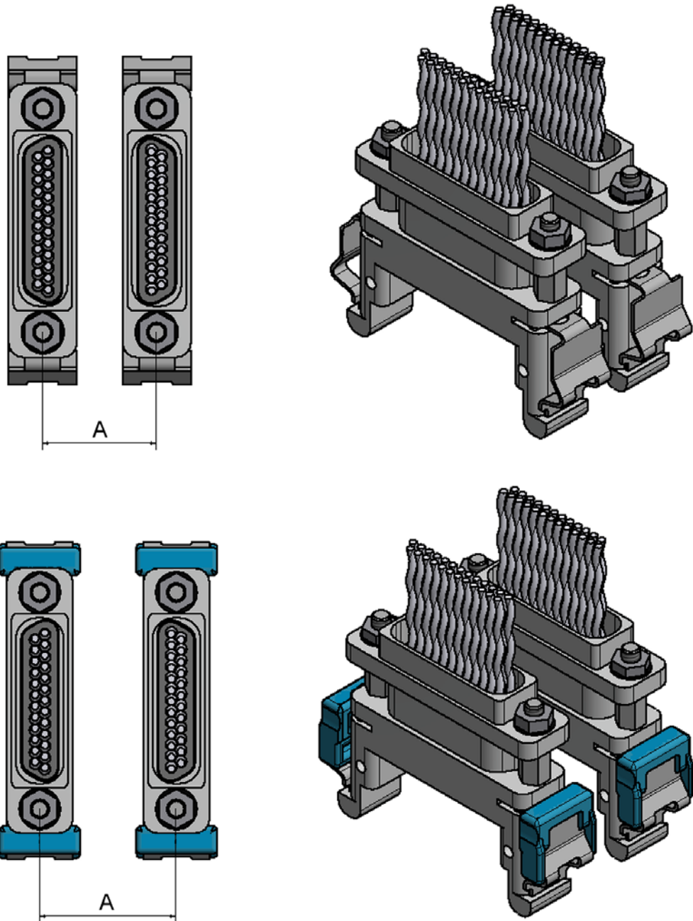
FIGURE 2.3.2 – VERTICAL RECOMMENDED SPACING
