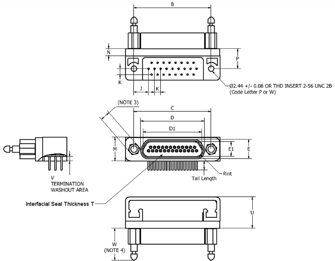
FIGURE 2.1L – VARIANT 06 – RECEPTACLE, FEMALE CONTACTS, 90° PCB (1.91mm) MOUNTING
