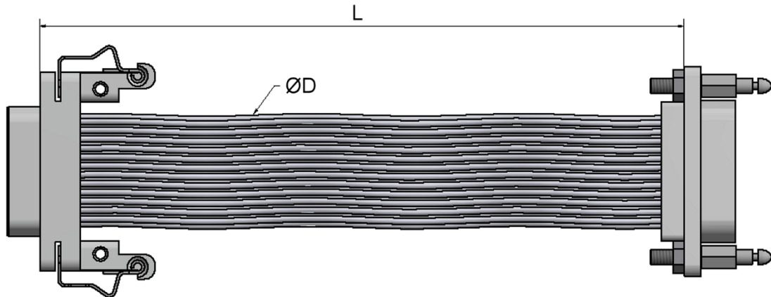
FIGURE 2.1M – VARIANT 07 – JUMPER, CONNECTOR 1: VARIANT 01, CONNECTOR 2: VARIANT 02
