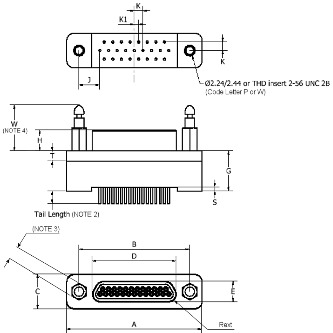
FIGURE 2.11 – VARIANT 05 – PLUG, MALE CONTACTS, STRAIGHT PCB (1.91mm) MOUNTING (CONNECTOR SHOWN WITH STANDARD LATCH POSTS)
