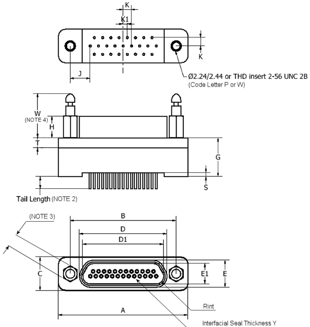
FIGURE 2.1J – VARIANT 05 – RECEPTACLE, FEMALE CONTACTS, STRAIGHT PCB (1.91mm) MOUNTING
