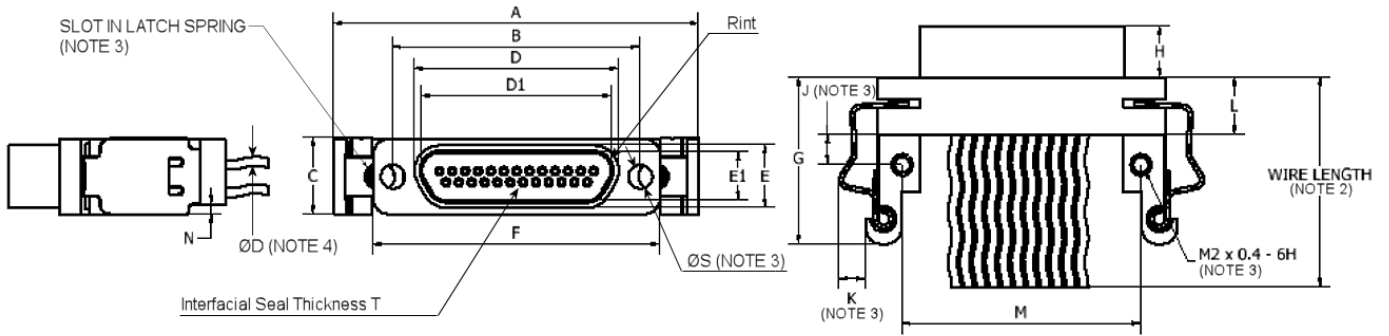
FIGURE 2.1B – VARIANT 01 – RECEPTACLE, FEMALE CONTACTS, PIGTAIL, LATCH SPRINGS
