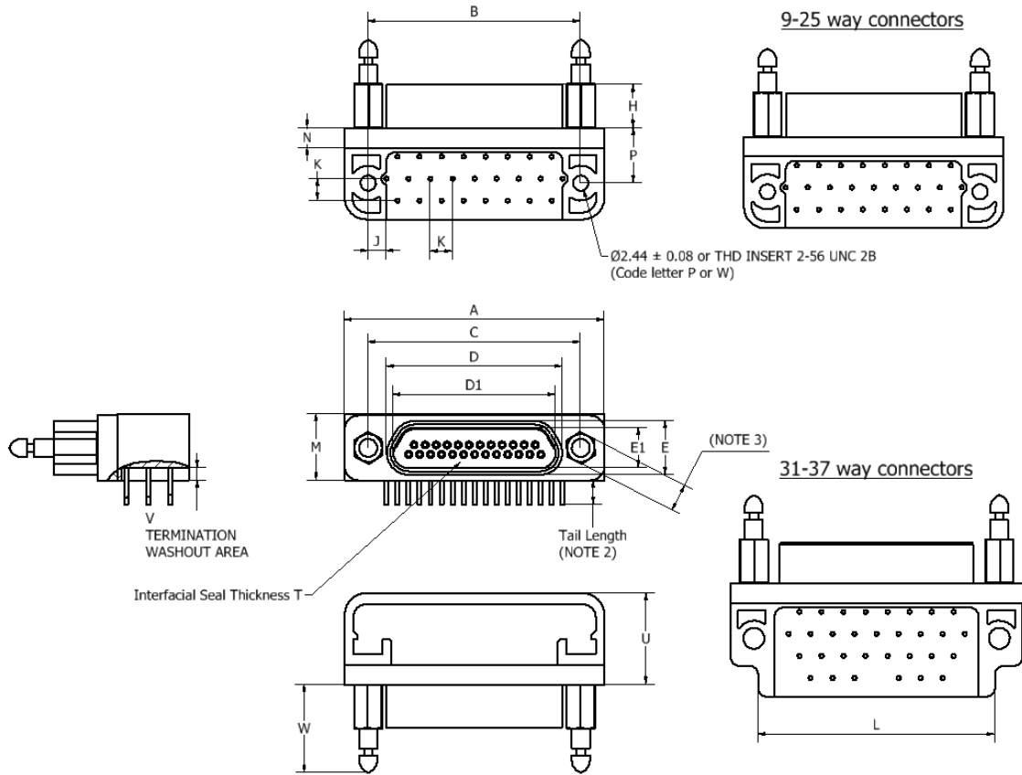
FIGURE 2.1F – VARIANT 03 – RECEPTACLE, FEMALE CONTACTS, 90° PCB (2.54mm) MOUNTING
