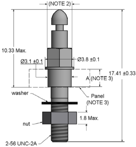
Panel-Mount Latch Post Applicable to Variants 02, 07, 09
