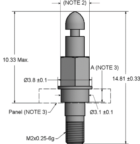
Panel-Mount Latch Post Applicable to Variants 03, 06
