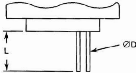
FIGURE 2.6 - UNINSULATED SOLID WIRE FOR PCB VARIANTS
