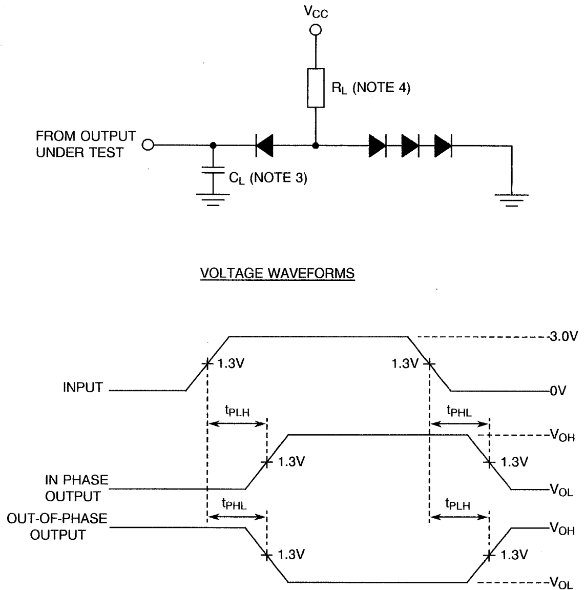
FIGURE 4(h) - DYNAMIC TEST AND SWITCHING WAVEFORMS
