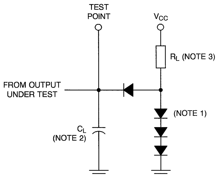
FIGURE 4(h) - DYNAMIC TEST AND SWITCHING WAVEFORMS
