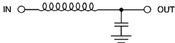
FIGURE 3 - FUNCTIONAL DIAGRAM
