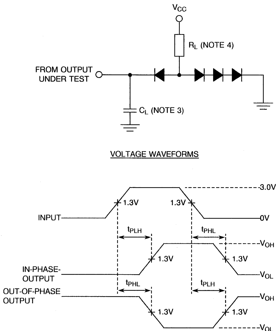
FIGURE 4(h) - DYNAMIC TEST AND SWITCHING WAVEFORMS
