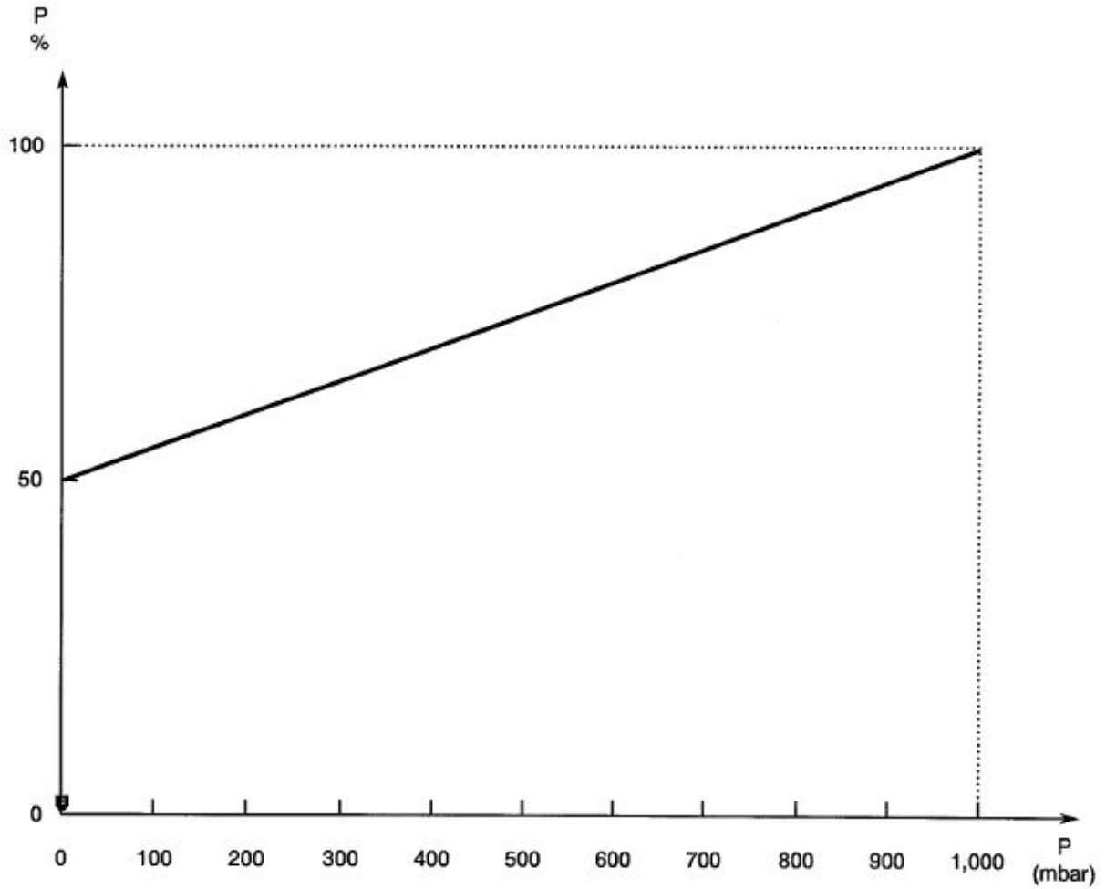
FIGURE 1(c) - POWER VERSUS PRESSURE
