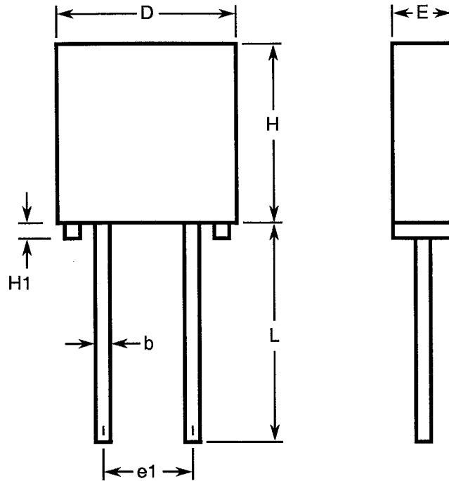
FIGURE 2 - PHYSICAL DIMENSIONS
