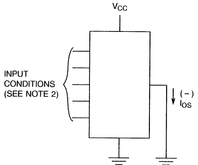
FIGURE 4(f) - SHORT CIRCUIT OUTPUT CURRENT
