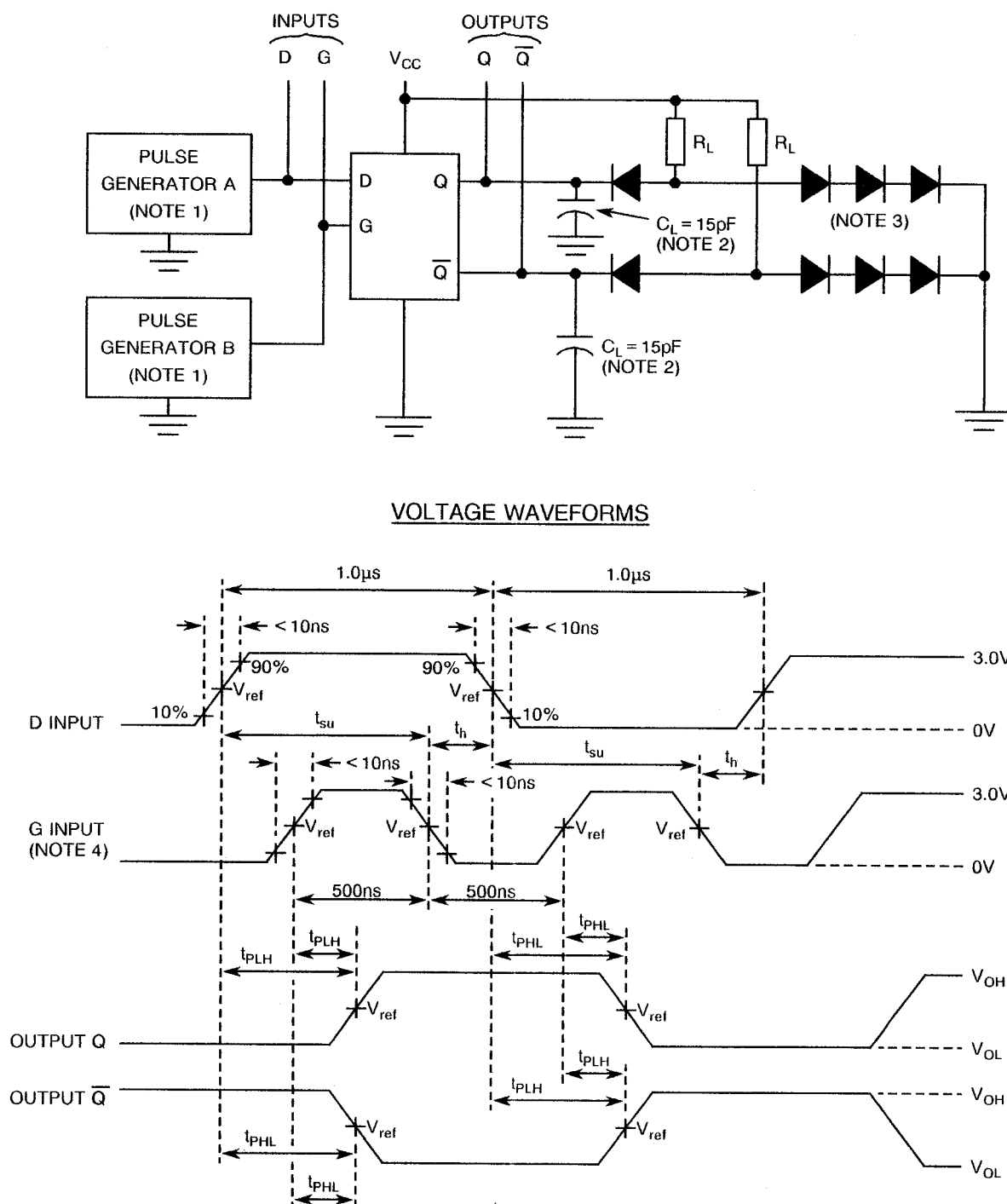
FIGURE 4(h) - DYNAMIC TEST AND SWITCHING WAVEFORMS
