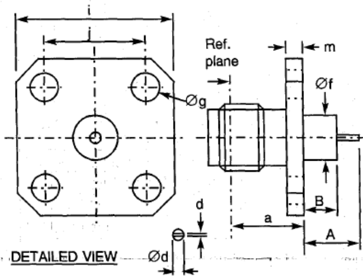
VARIANT 45 – SQUARE FLANGE RECEPTACLE FOR MICRO-STRIP
