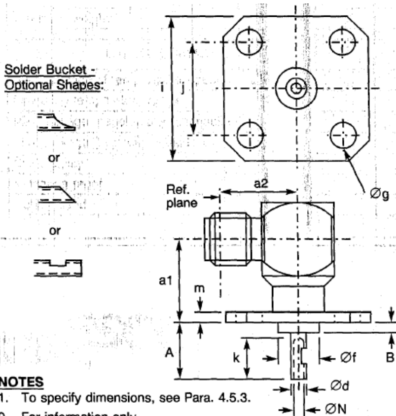
VARIANT 28 - ELBOW RECEPTACLE, SQUARE FLANGE
