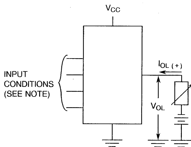
FIGURE 4(d) - HIGH LEVEL OUTPUT VOLTAGE
