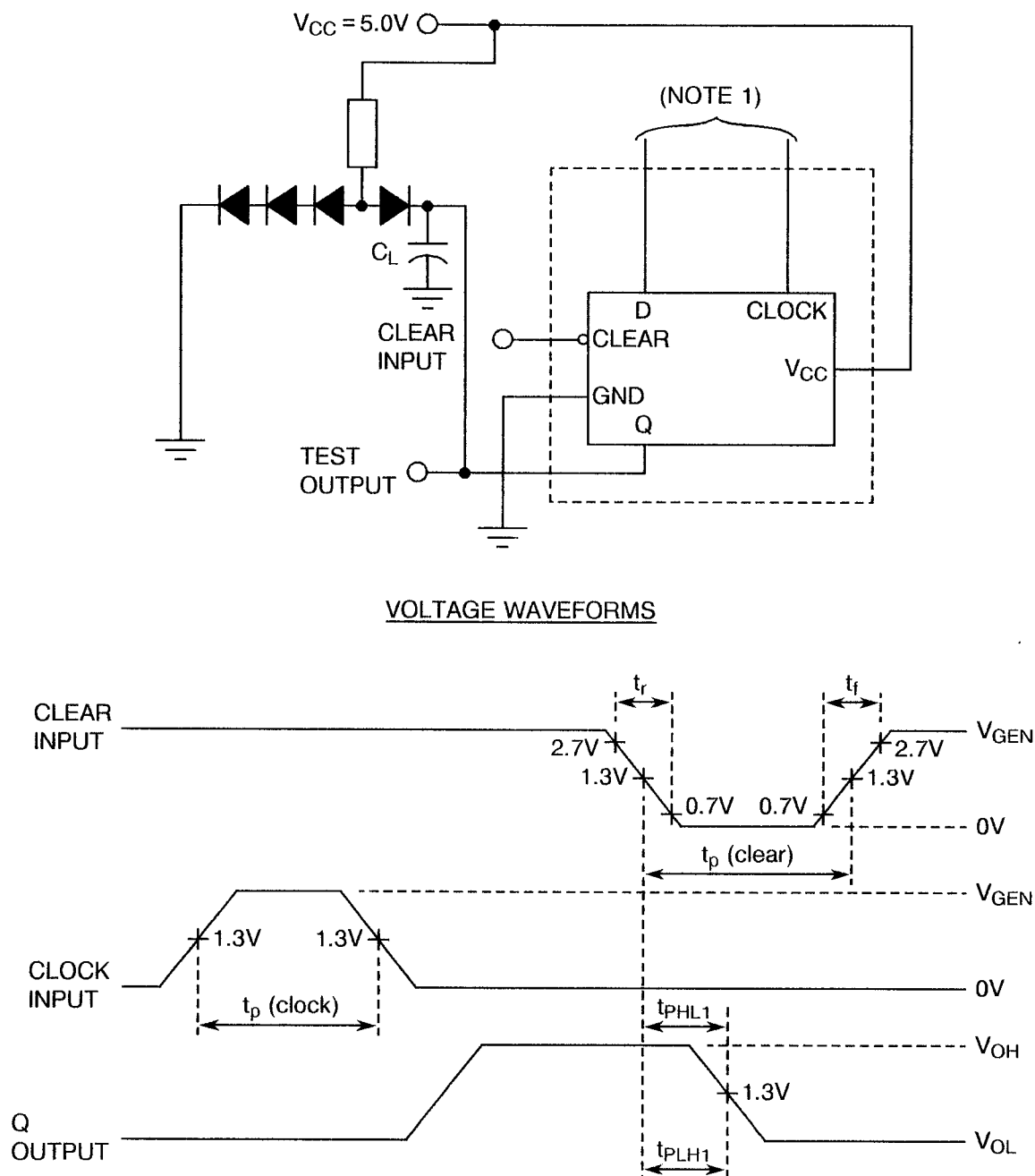
FIGURE 4(h) - DYNAMIC TEST AND SWITCHING WAVEFORMS
