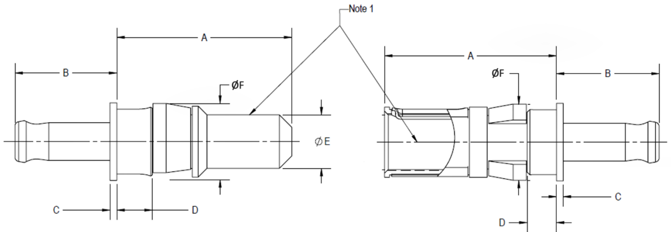
FIGURE 2(a) – POWER PRESS-FIT CONTACTS, MALE AND FEMALE
