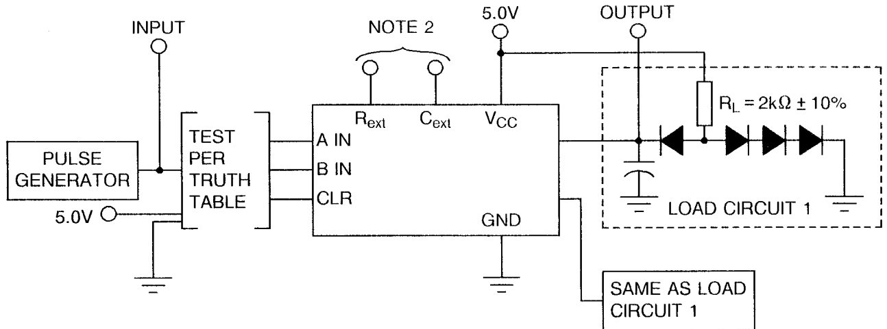
FIGURE 4(h) - DYNAMIC TEST AND SWITCHING WAVEFORMS
