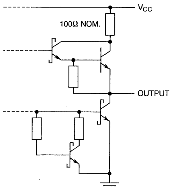
TYPICAL OF ALL OUTPUTS
