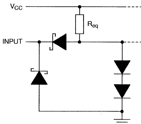
EQUIVALENT OF EACH INPUT
