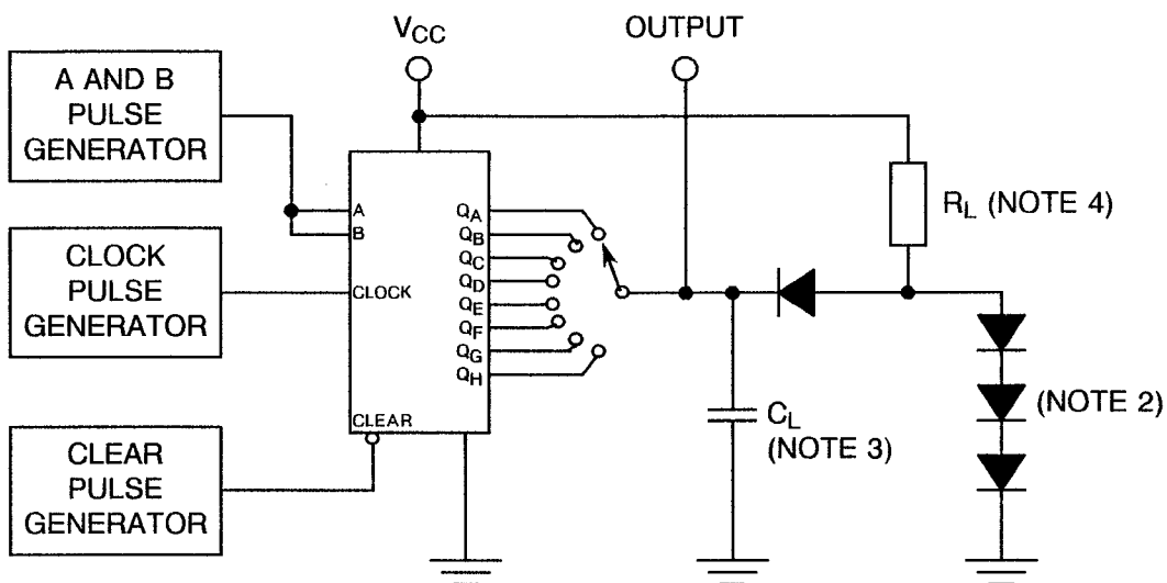
FIGURE 4(h) - DYNAMIC TEST AND SWITCHING WAVEFORMS
