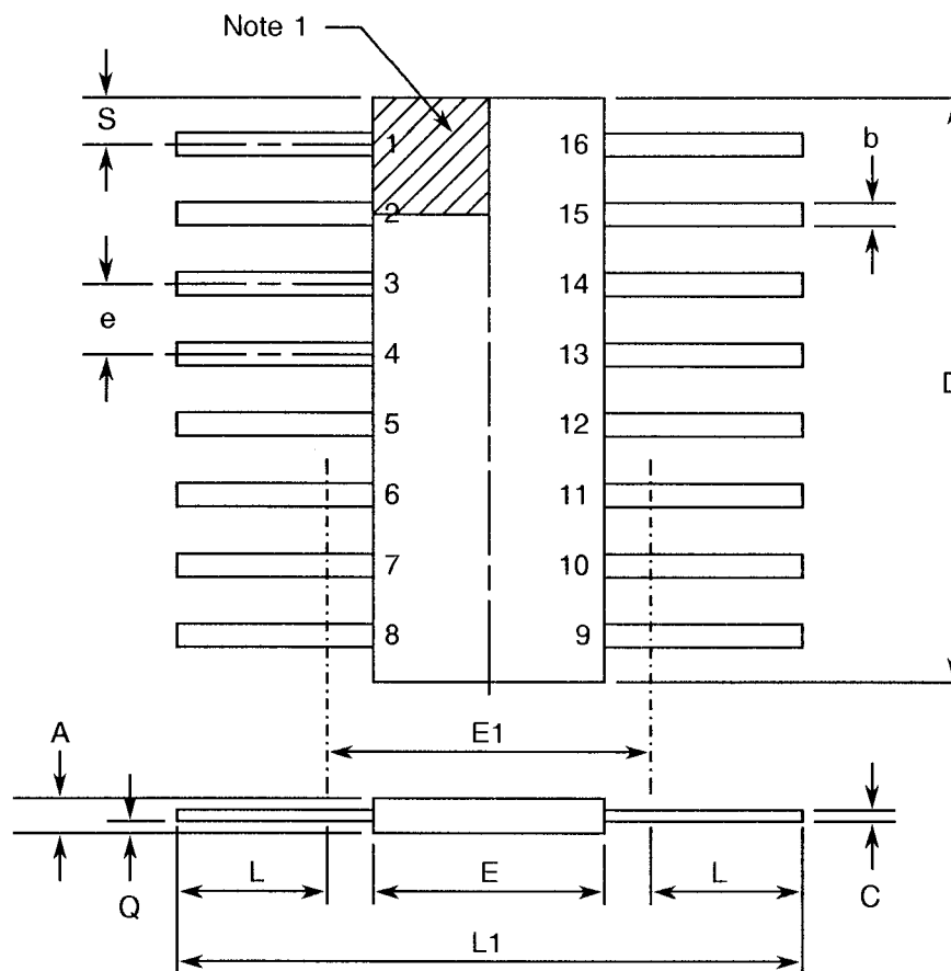
FIGURE 2(a) - FLAT PACKAGE
