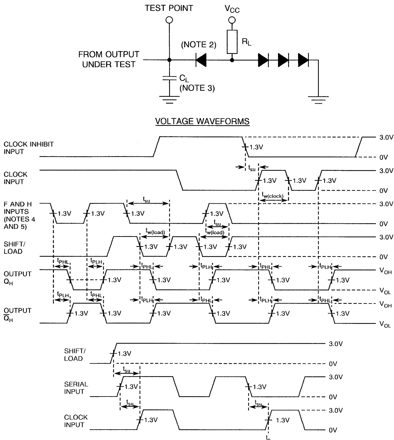
FIGURE 4(h) - DYNAMIC TEST AND SWITCHING WAVEFORMS
