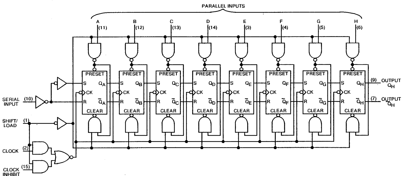
FIGURE 3(d) - FUNCTIONAL DIAGRAM
