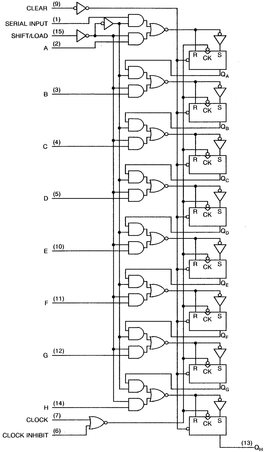
FIGURE 3(d) - FUNCTIONAL DIAGRAM
