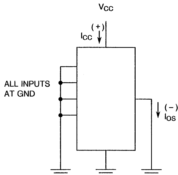
FIGURE 4(f) - SHORT CIRCUIT OUTPUT CURRENT
