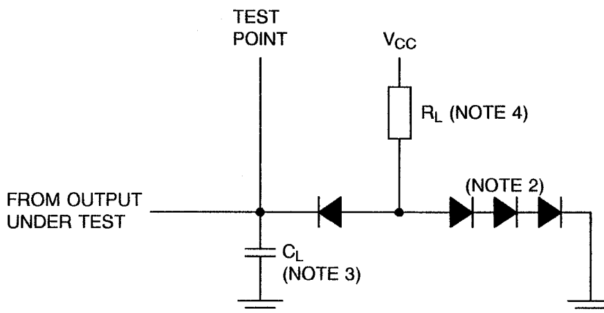
FIGURE 4(h) - DYNAMIC TEST AND SWITCHING WAVEFORMS
