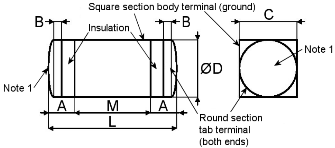
FIGURE 2 – PHYSICAL DIMENSIONS
