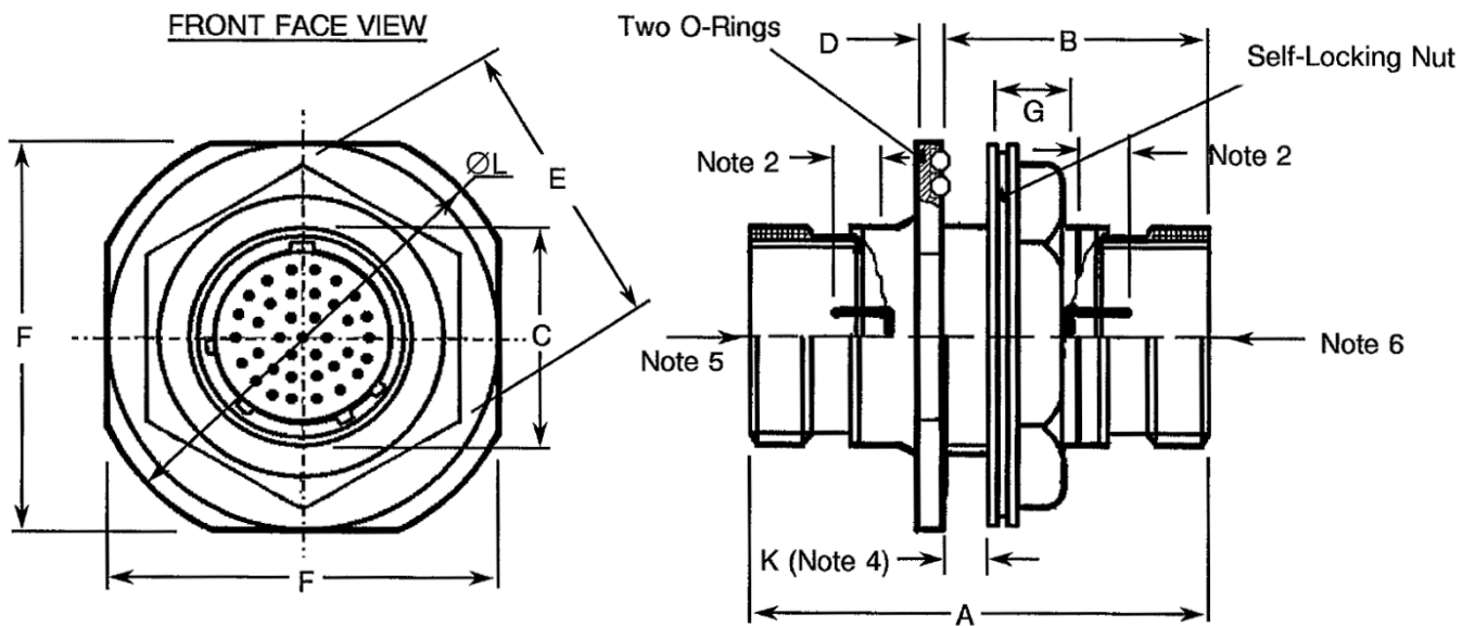
FIGURE 2(a) – RECEPTACLES (CONTINUED)
