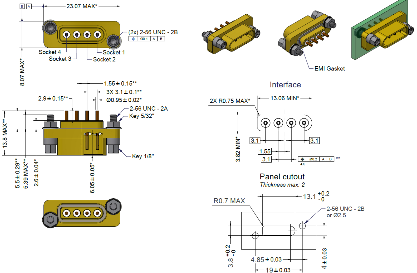
FIGURE 2(d) – VARIANT 04 - SPACEFIBRE HDR, FEMALE, PANEL MOUNT RECEPTACLE WITH PIN PCB TERMINATIONS
