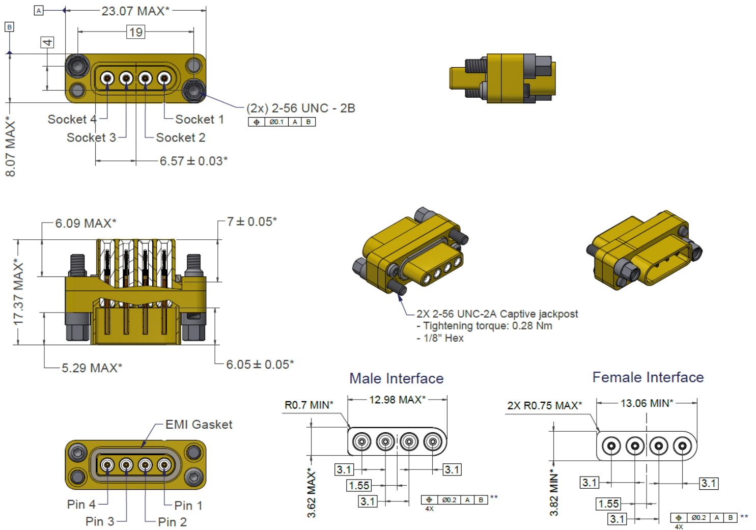
FIGURE 2(g) – VARIANT 07 - CONNECTOR SAVER, SPACEFIBRE HDR
