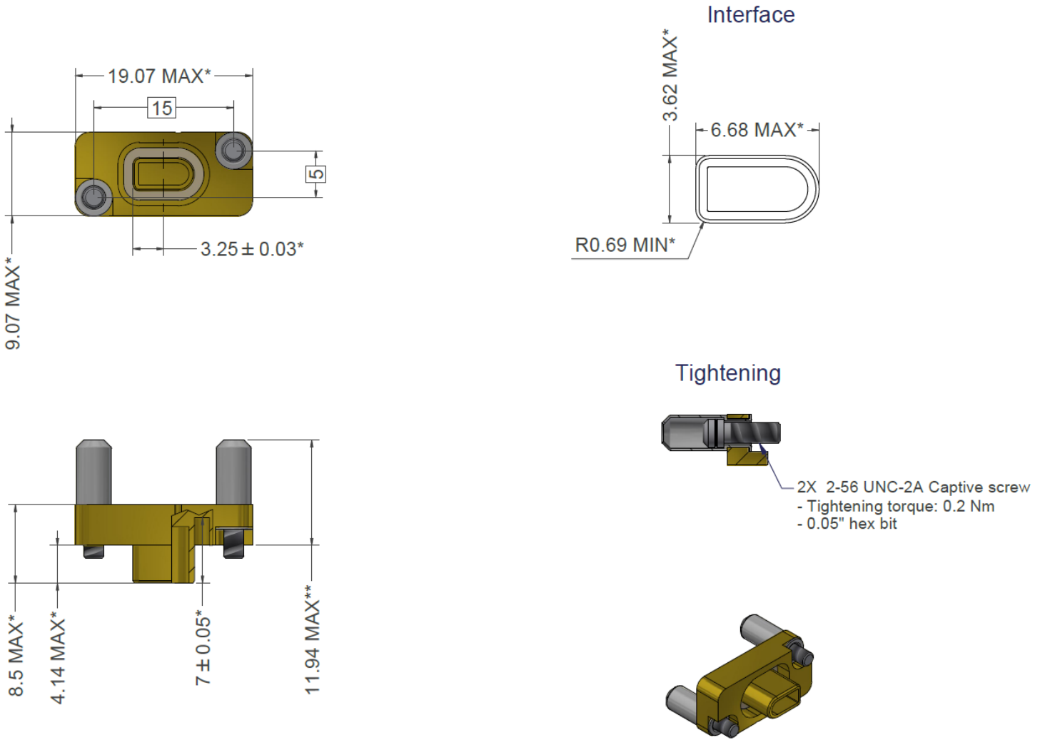
FIGURE 2(d) – VARIANT 04 - BLANKING PLUG, AXOMACH HDR, 1 WAY
