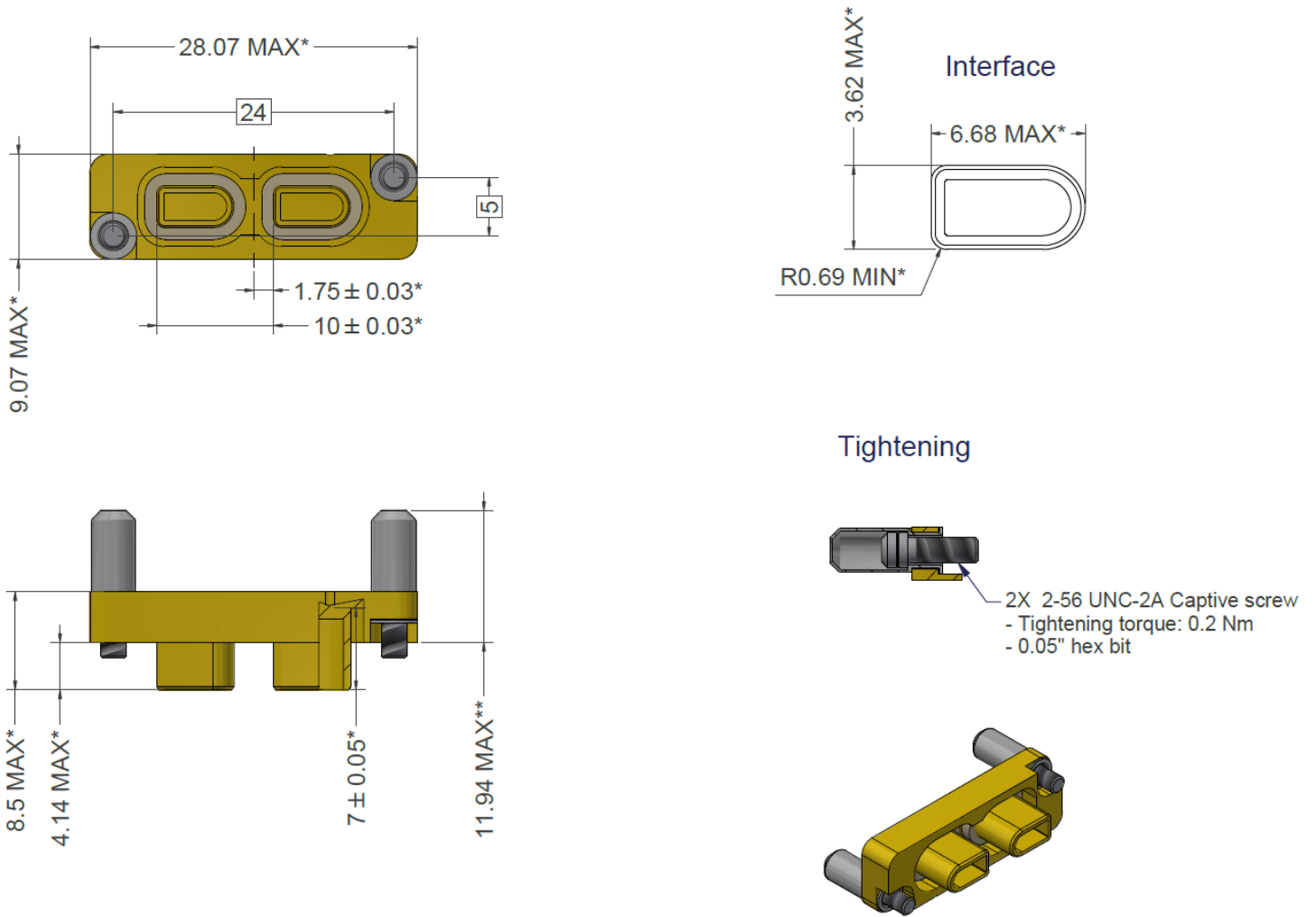
FIGURE 2(e) – VARIANT 05 - BLANKING PLUG, AXOMACH HDR, 2 WAY
