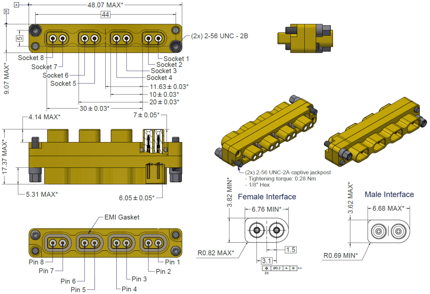
FIGURE 2(c) – VARIANT 03 - CONNECTOR SAVER, AXOMACH HDR, 4 WAY
