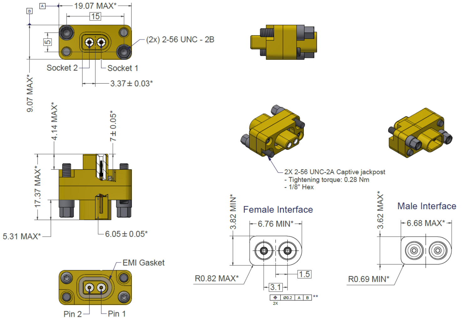
FIGURE 2(a) – VARIANT 01 - CONNECTOR SAVER, AXOMACH HDR, 1 WAY
