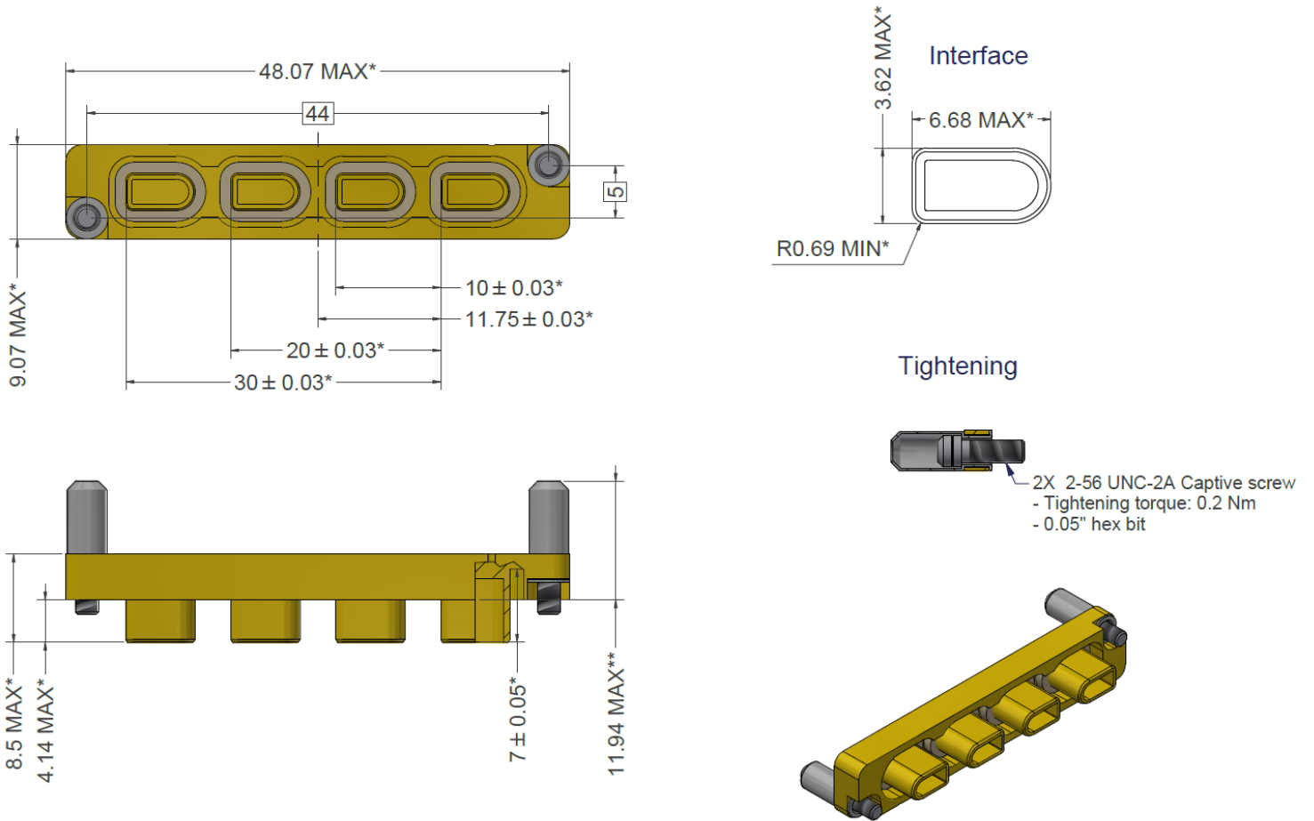
FIGURE 2(f) – VARIANT 06 - BLANKING PLUG, AXOMACH HDR, 4 WAY
