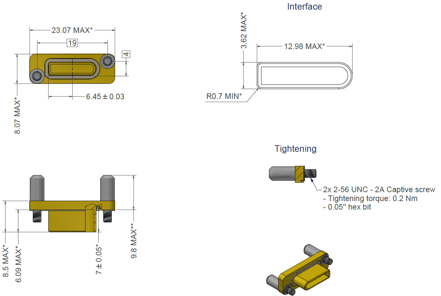
FIGURE 2(h) – VARIANT 08 - BLANKING PLUG, SPACEFIBRE HDR
