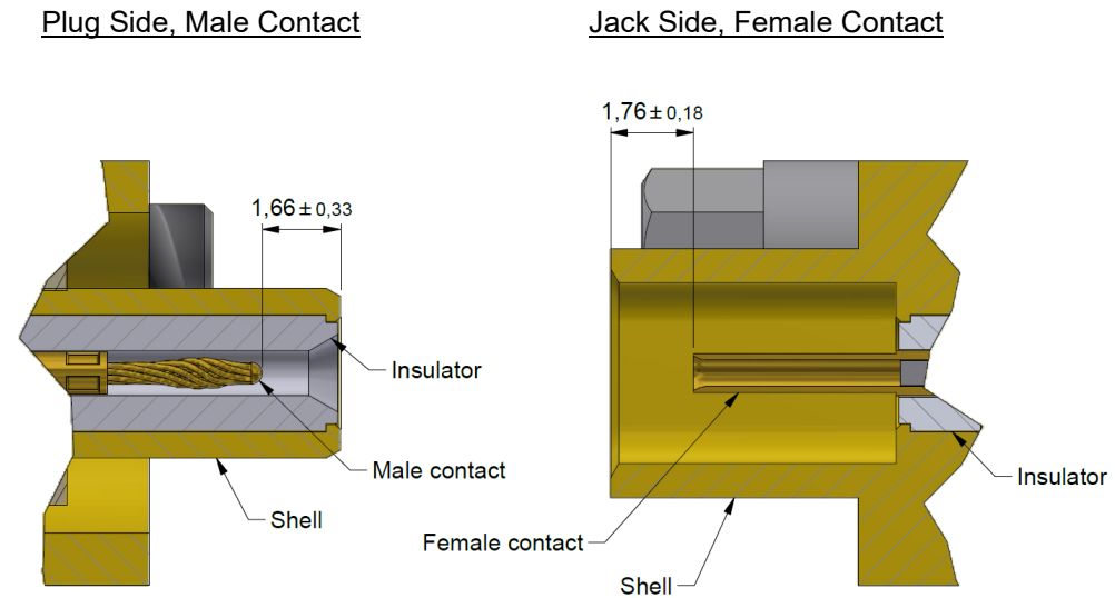
FIGURE 2(h) - INTERFACE DIMENSIONS – VARIANTS 01, 02, 03, 07
