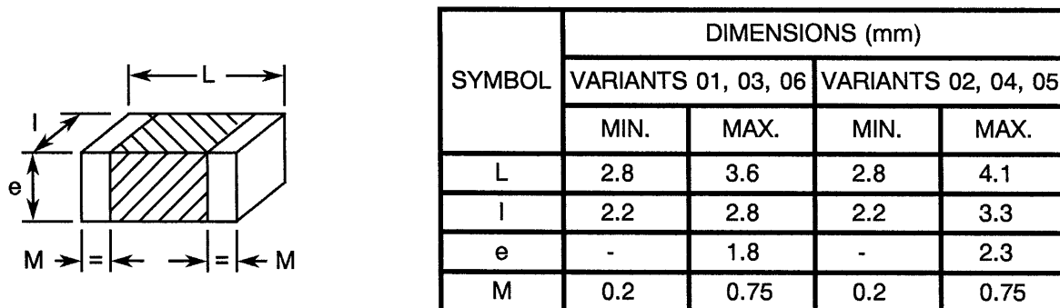
FIGURE 2 - PHYSICAL DIMENSIONS
