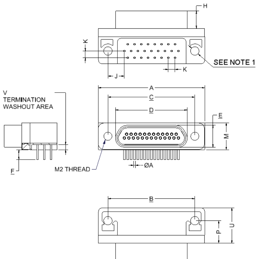
FIGURE 2.2Z - CONNECTORS TYPE – 75RBB AND 75RBT
