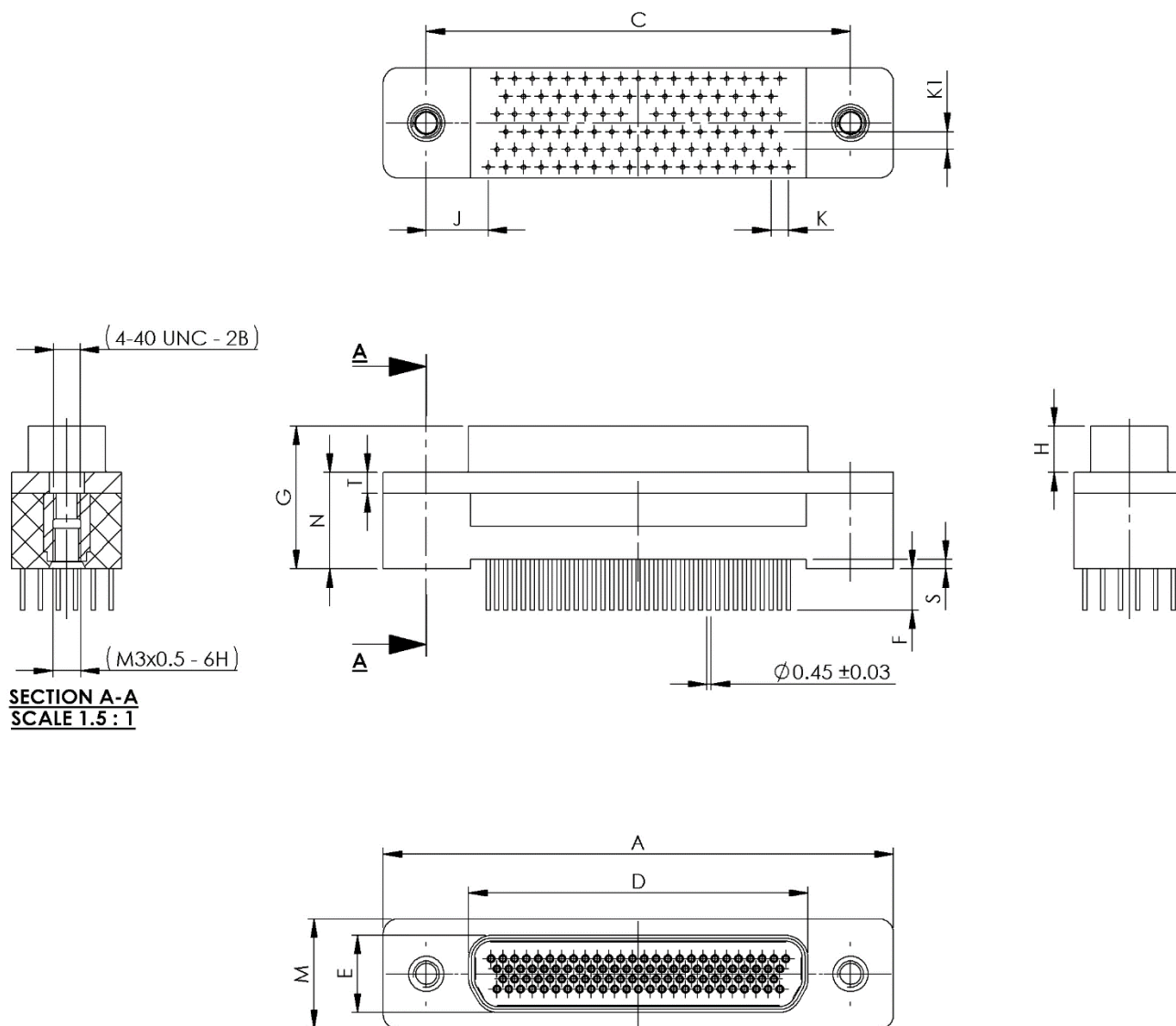
FIGURE 2.2X - CONNECTORS TYPE – GMR7580
