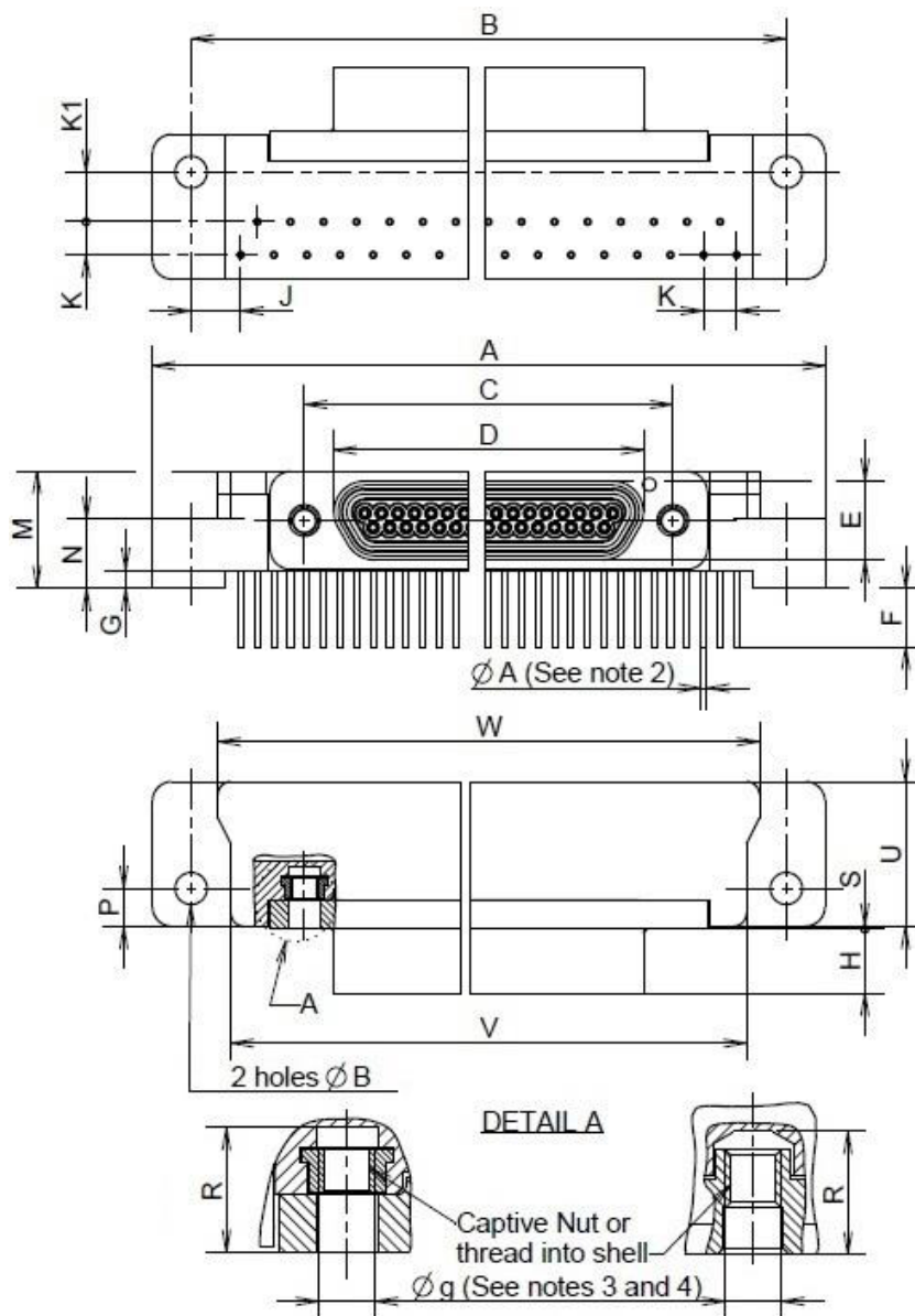
FIGURE 2.2B - CONNECTORS TYPE - FR136
