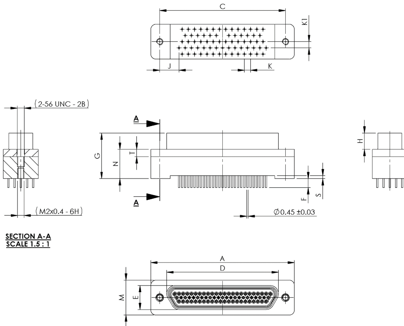
FIGURE 2.2V - CONNECTORS TYPE – GMR7580
