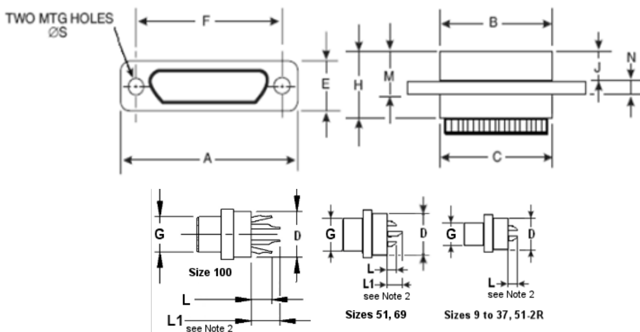
FIGURE 2.2L CONNECTORS TYPE FR164 - RECEPTACLE FEMALE CONTACTS
