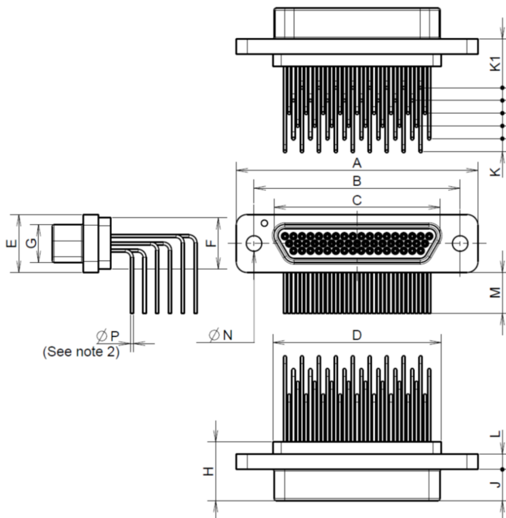
FIGURE 2.2AQ - CONNECTORS TYPE – FR171
