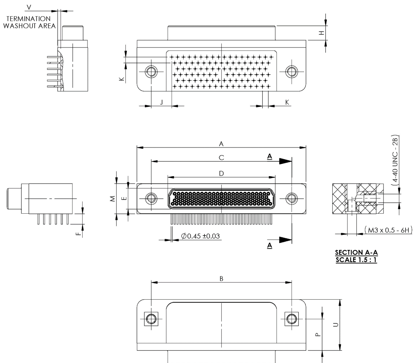
FIGURE 2.2Q - CONNECTORS TYPE – GMR7590
