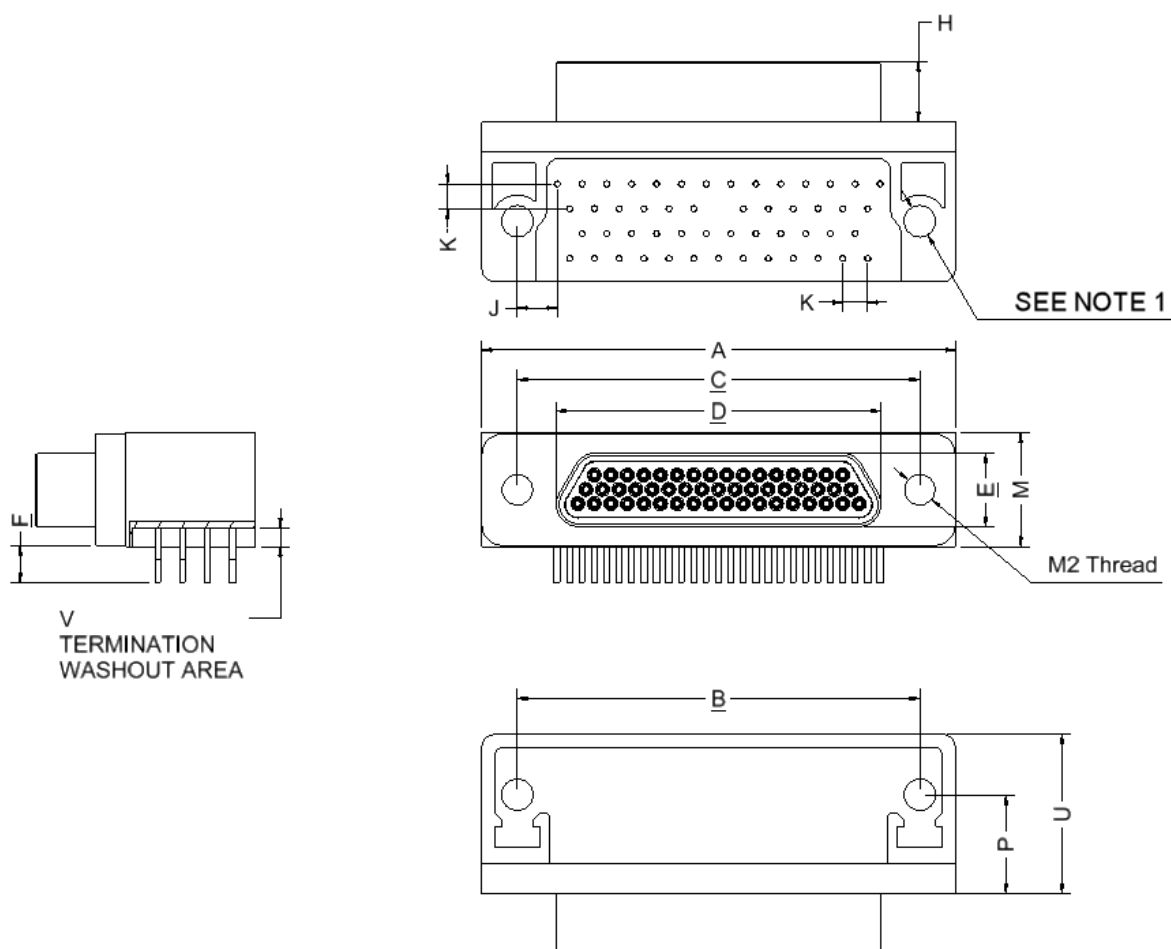
FIGURE 2.2AA - CONNECTORS TYPE – 75RBB AND 75RBT
