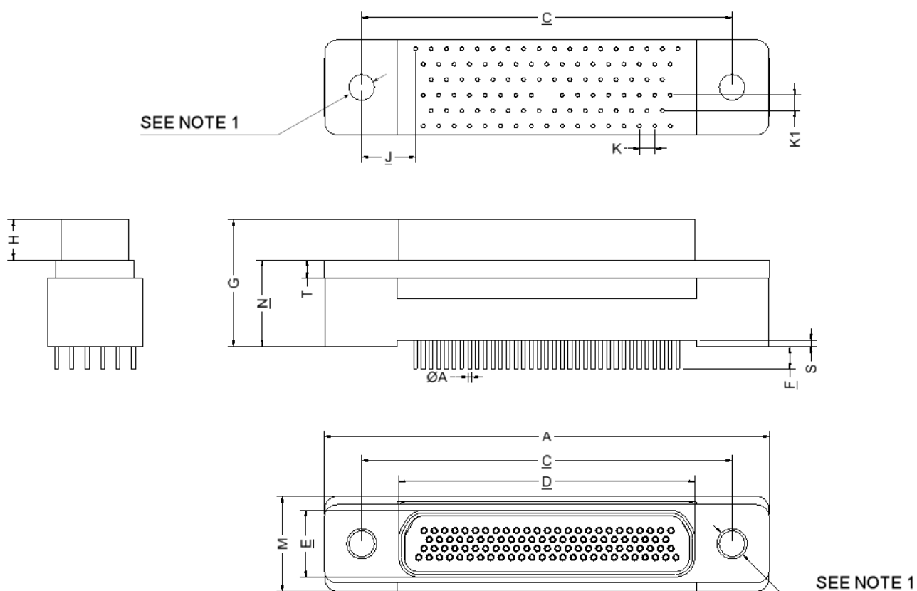
FIGURE 2.2AJ - CONNECTORS TYPE – 75SBB AND 75SBT
