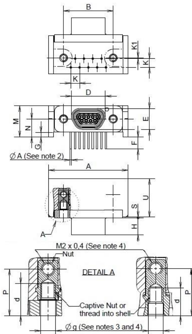
FIGURE 2.2F - CONNECTORS TYPE - FR136A
