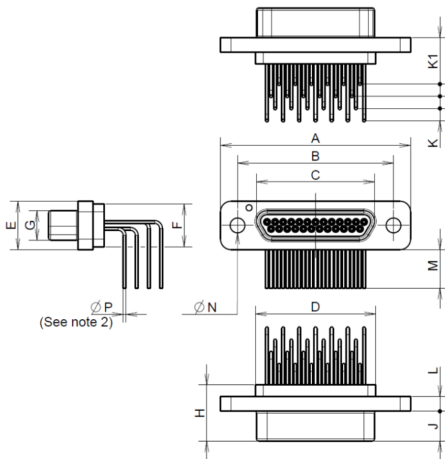
FIGURE 2.2AO - CONNECTORS TYPE – FR171
