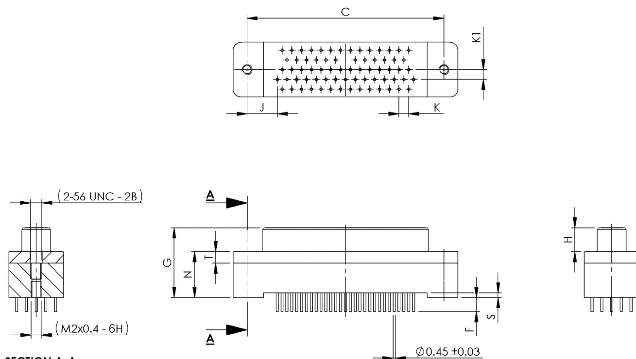
FIGURE 2.2U - CONNECTORS TYPE – GMR7580
