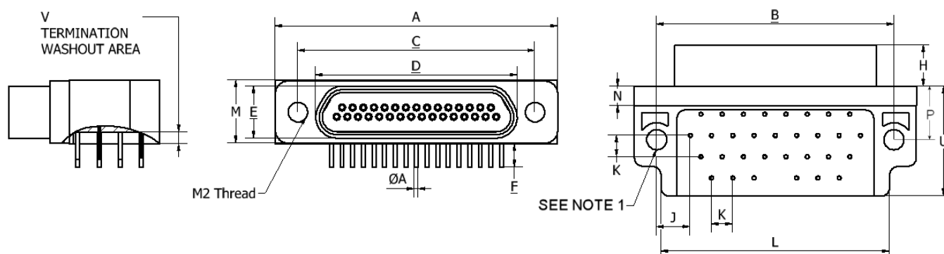
FIGURE 2.2AN - CONNECTORS TYPE – CBRB AND CBRT
