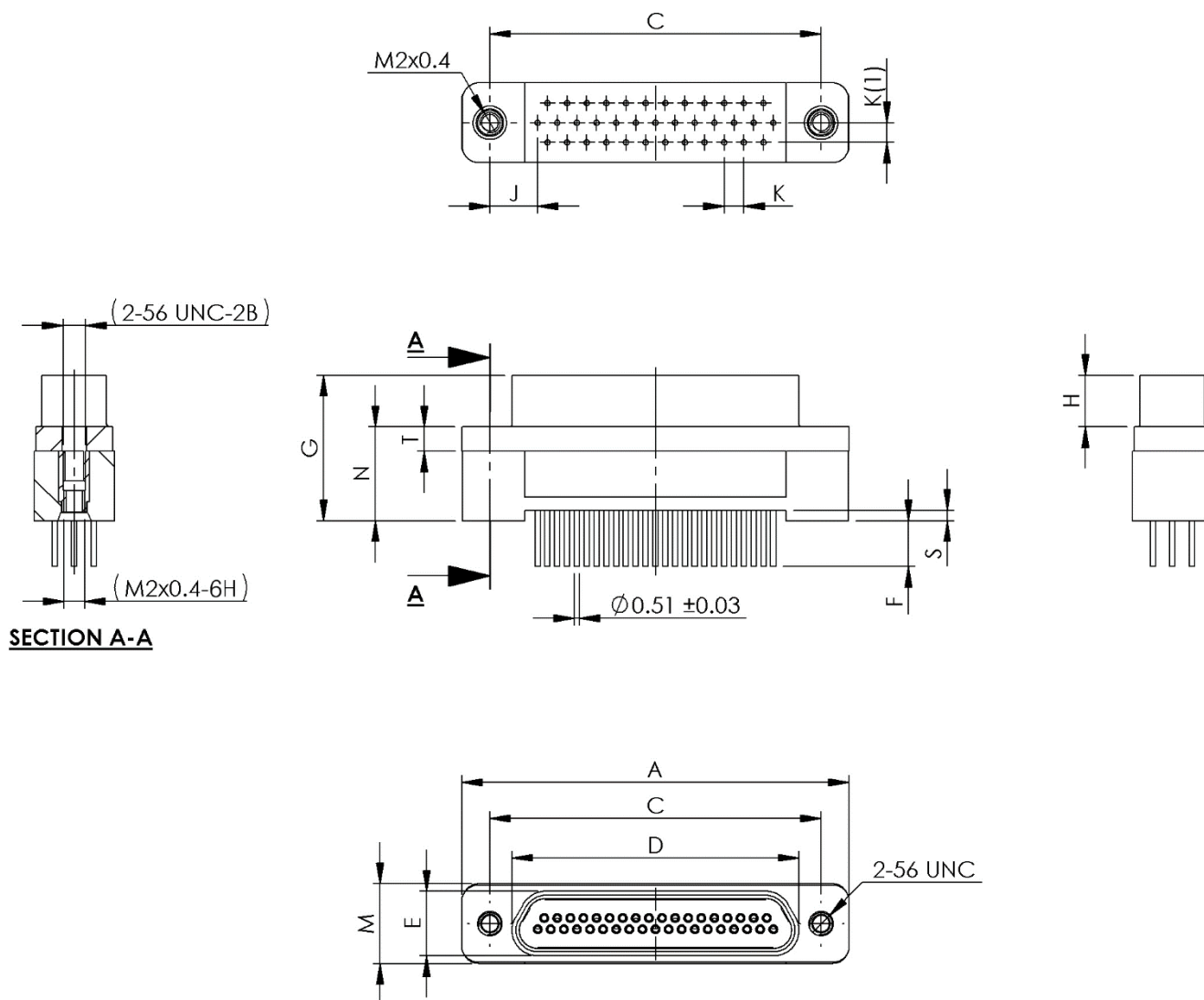
FIGURE 2.2T - CONNECTORS TYPE – GMR7580
