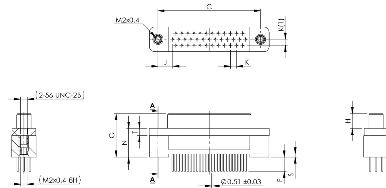
FIGURE 2.2S - CONNECTORS TYPE – GMR7580
