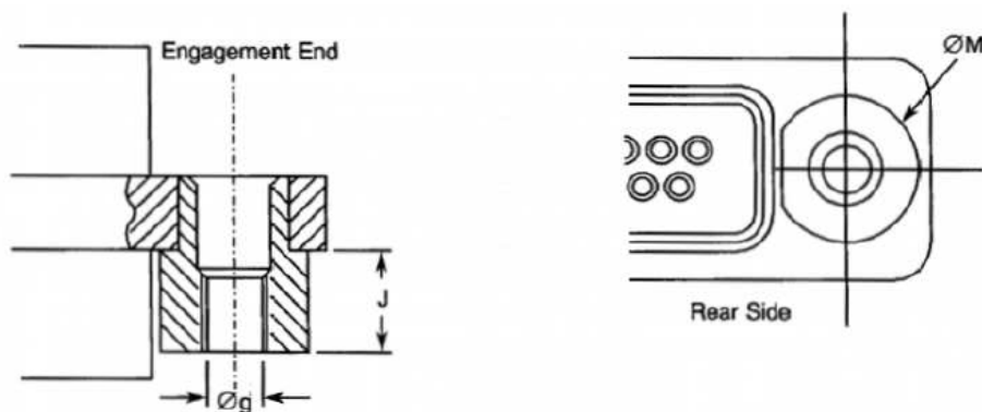
FIGURE 2.8 - CAPTIVE NUT
