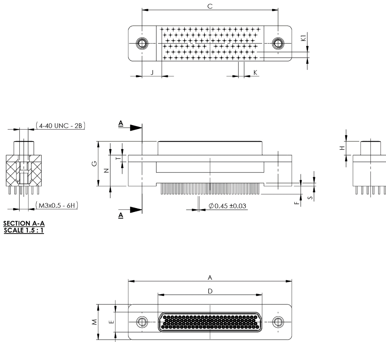
FIGURE 2.2W - CONNECTORS TYPE – GMR7580
