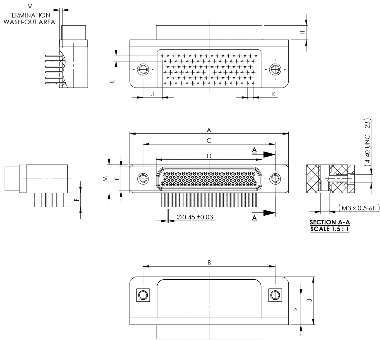
FIGURE 2.2R - CONNECTORS TYPE – GMR7590
