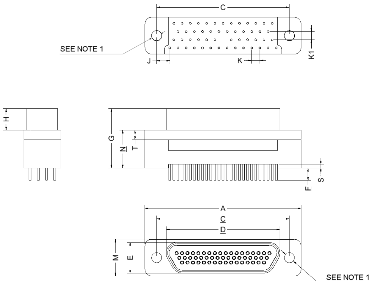
FIGURE 2.2AH - CONNECTORS TYPE – 75SBB AND 75SBT
