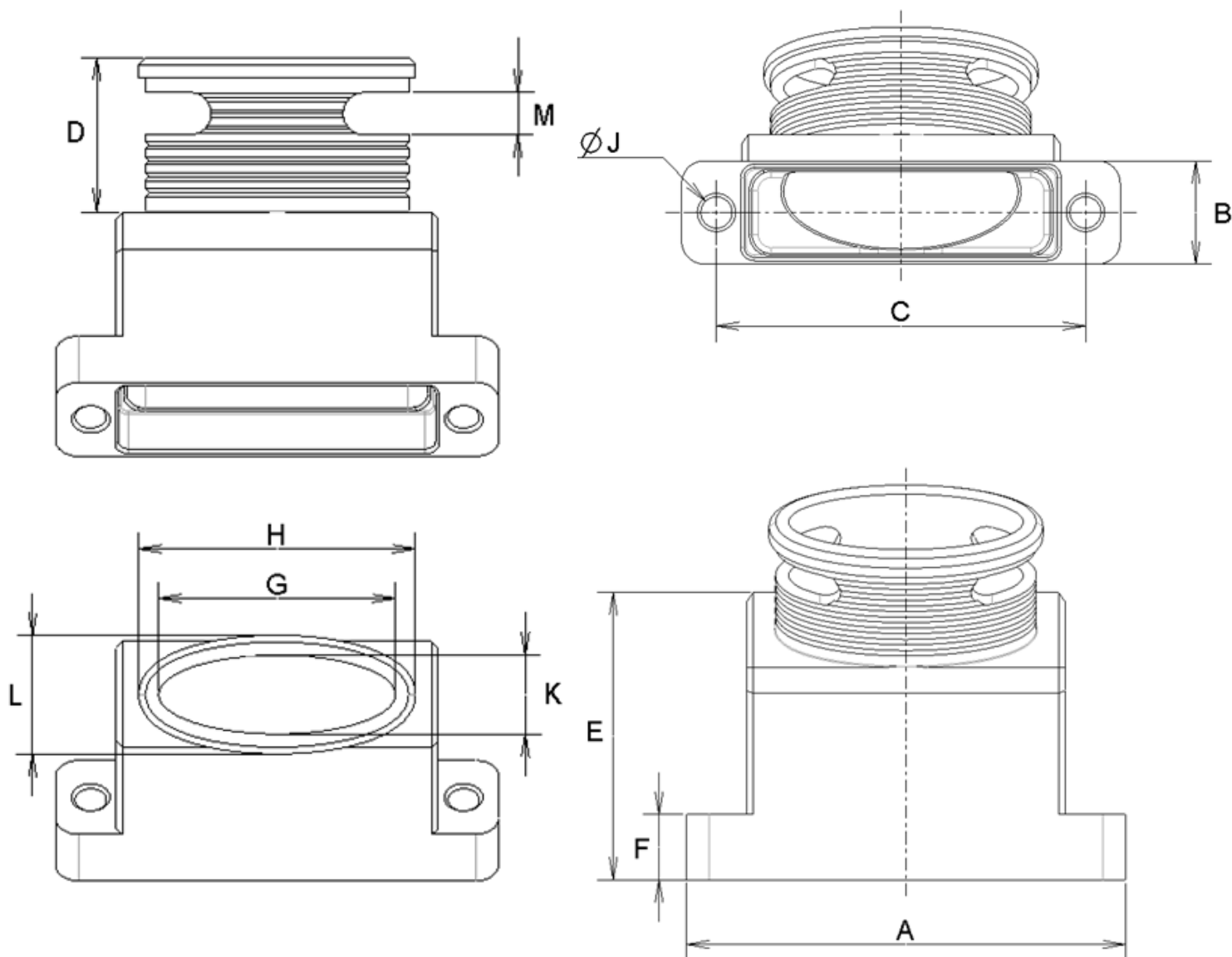
FIGURE 2(i) – BACKSHELL - LIGHTWEIGHT 45° FRONT ELLIPTICAL ENTRY
