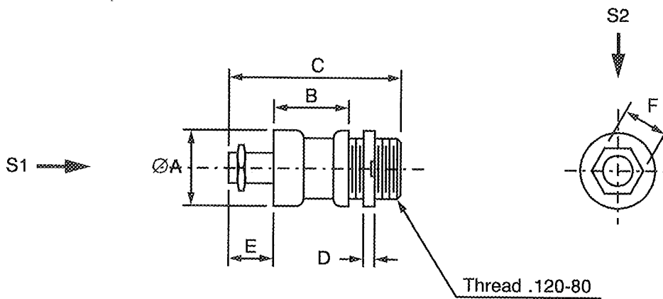
FIGURE 2(a) - VARIANT 01, LUG PANEL MOUNT
