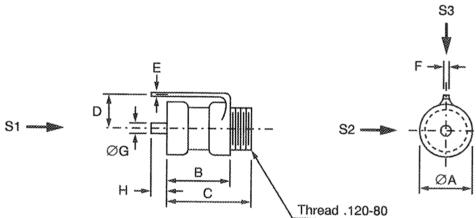
FIGURE 2(d) - VARIANT 04, VERTICAL MOUNT
