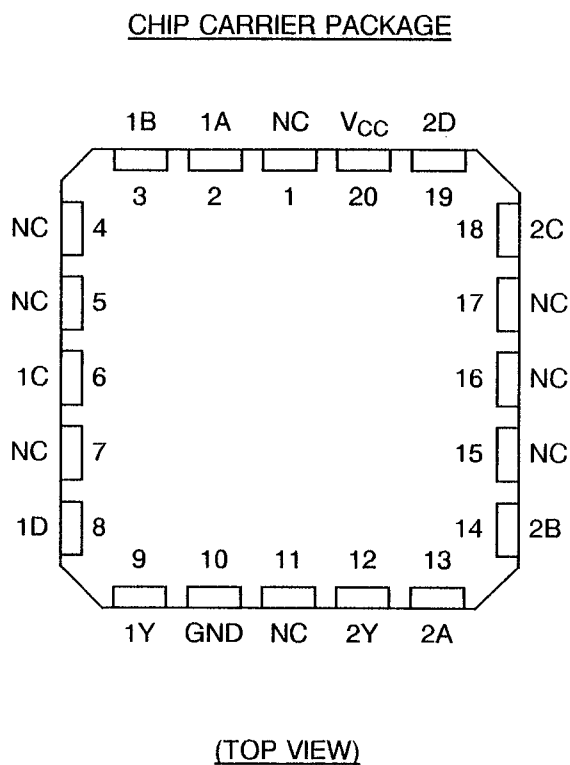
FIGURE 3(a) - PIN ASSIGNMENT
