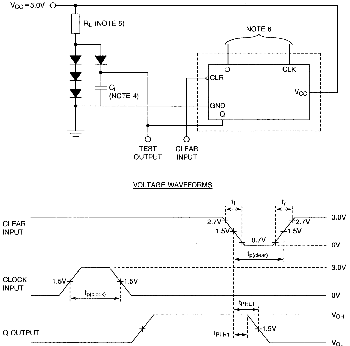
FIGURE 4(h) - DYNAMIC TEST AND SWITCHING WAVEFORMS
