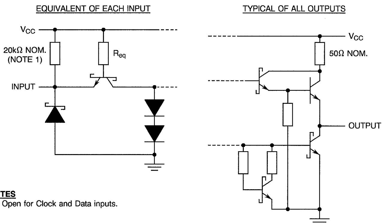
FIGURE 3(c) - CIRCUIT SCHEMATIC
