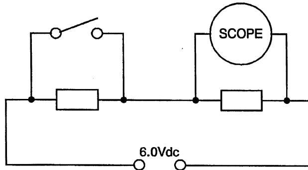
FIGURE 1B - TYPICAL OSCILLOSCOPE RECORDING FOR NON-INVERTER SWITCHES
