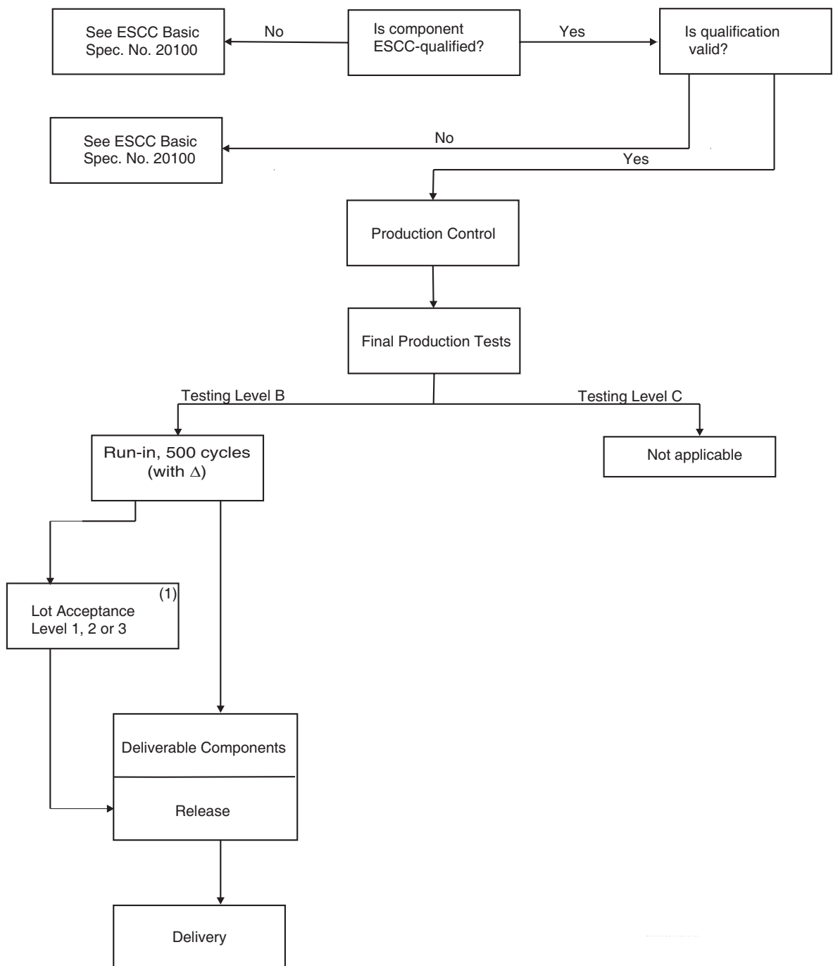
CHART I - TESTING LEVELS
