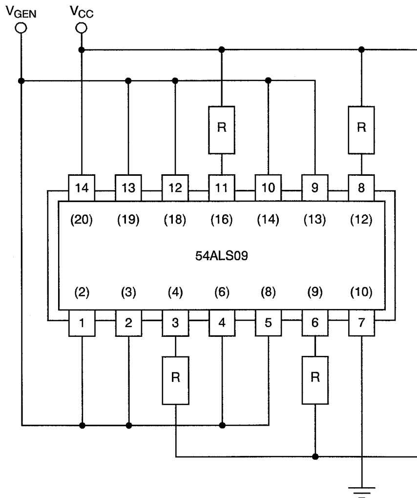
FIGURE 5 - ELECTRICAL CIRCUIT FOR POWER BURN-IN AND OPERATING LIFE TEST
