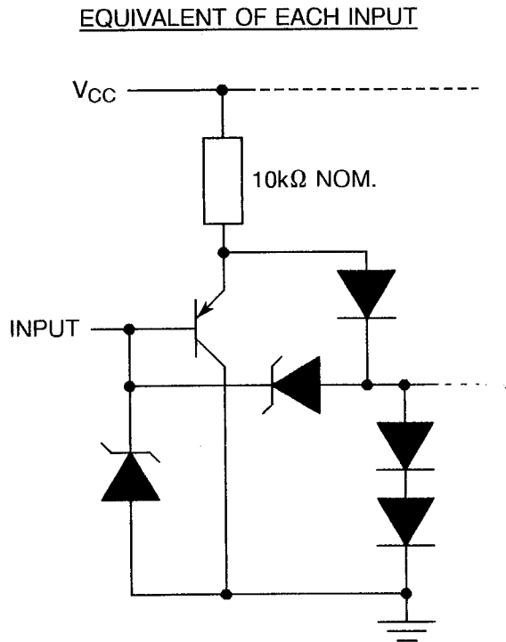
FIGURE 3(c) - CIRCUIT SCHEMATIC
