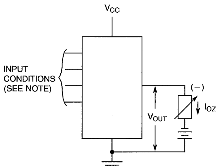
FIGURE 4(g) - OFF STATE OUTPUT CURRENT
