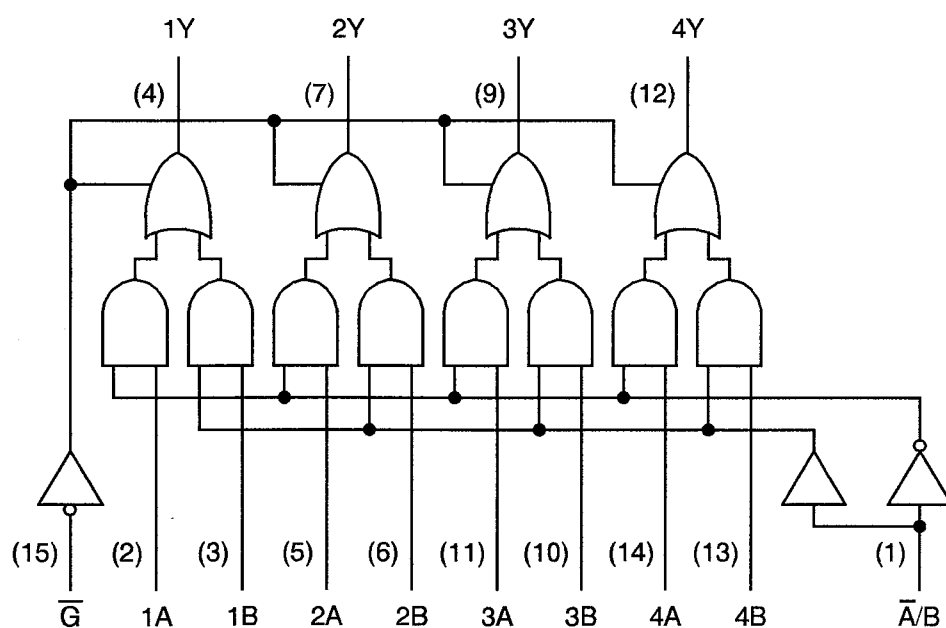
FIGURE 3(d) - FUNCTIONAL DIAGRAM
