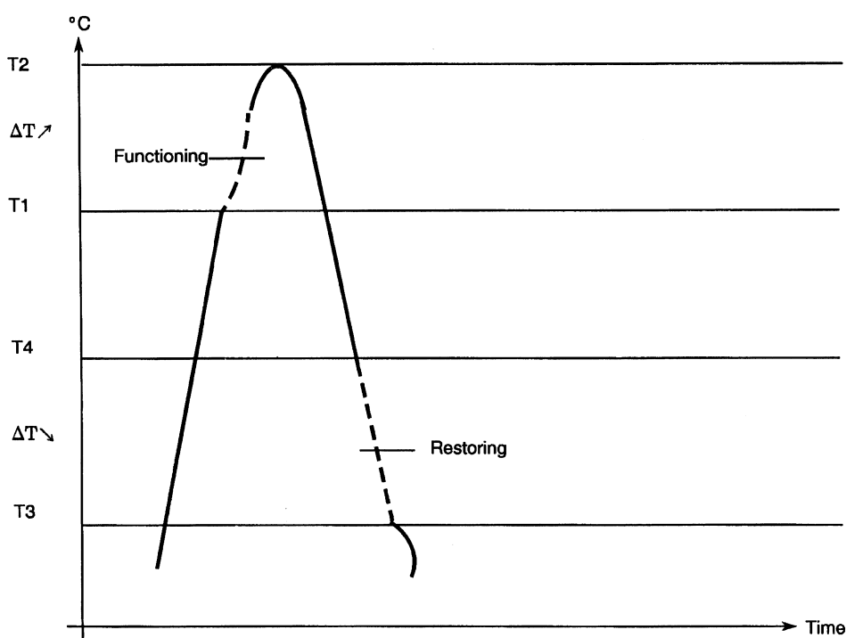
FIGURE III - THERMAL DIAGRAM FOR RUN-IN TEST
