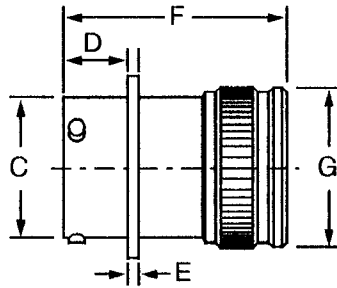
FIGURE 2 - PHYSICAL DIMENSIONS
