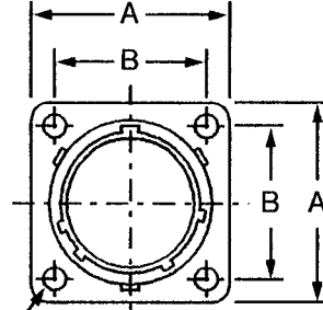
FIGURE 2 - PHYSICAL DIMENSIONS
