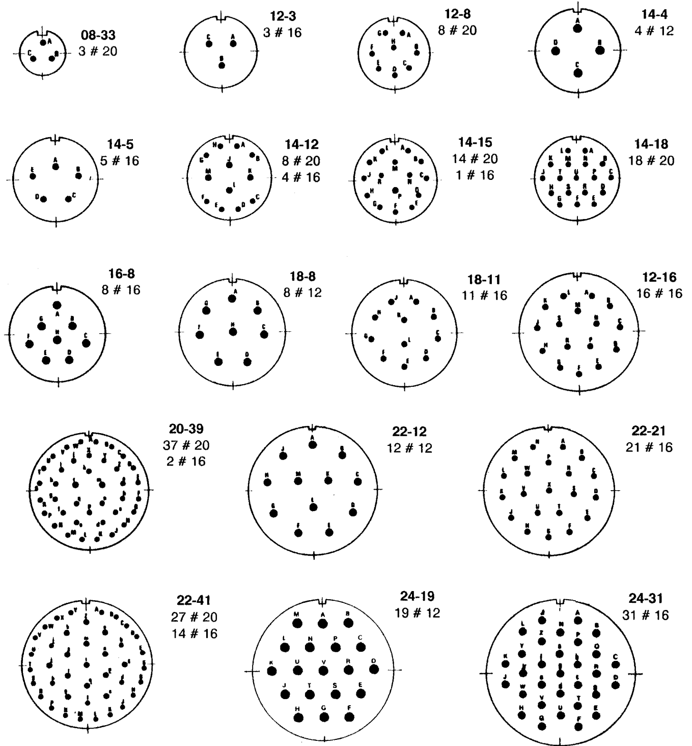
FIGURE 2(b) - STANDARD CONTACT ARRANGEMENTS - FRONT VIEW PIN INSERT (See Para. 4.5 for definition of numbers)
