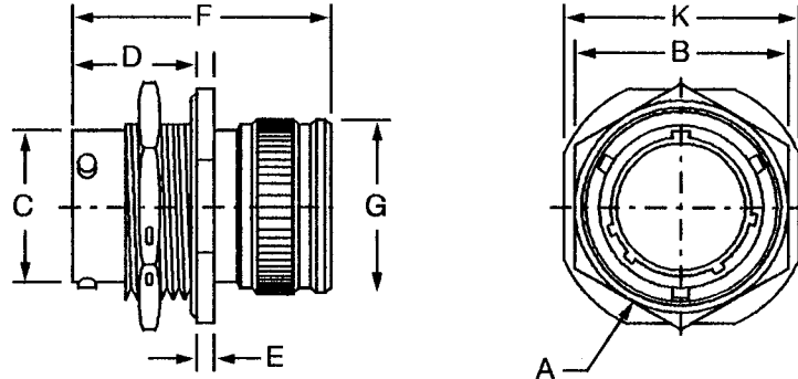
FIGURE 2 - PHYSICAL DIMENSIONS (CONTINUED)
