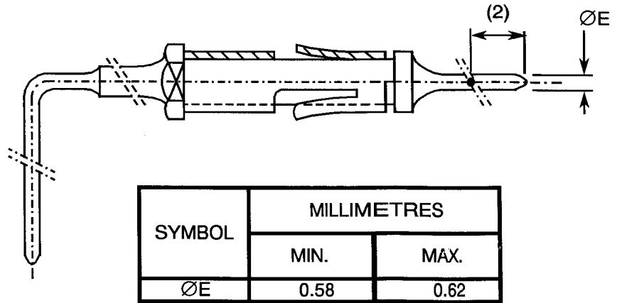
VARIANT 04 - CRIMP MALE CONTACT
