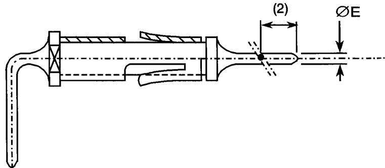
VARIANT 64 - SOLDER RIGHT-ANGLE MALE CONTACT (LONG)
