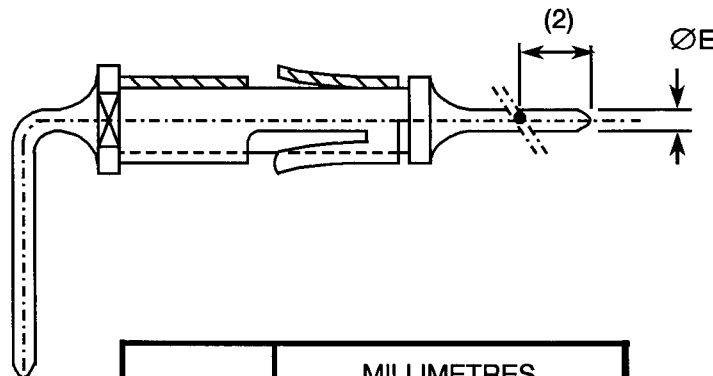
VARIANT 65 - SOLDER RIGHT-ANGLE MALE CONTACT (LONG)
