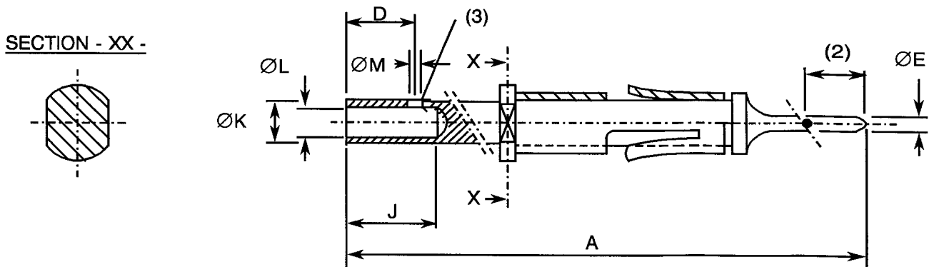
VARIANT 04 - CRIMP MALE CONTACT
