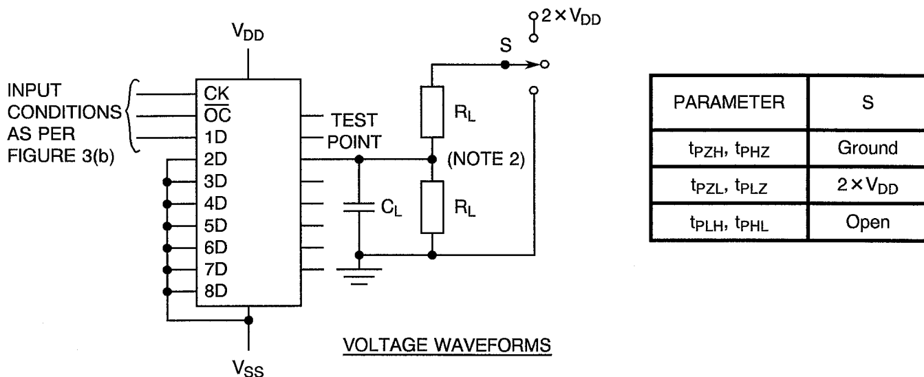
FIGURE 4(i) - PROPAGATION DELAY
