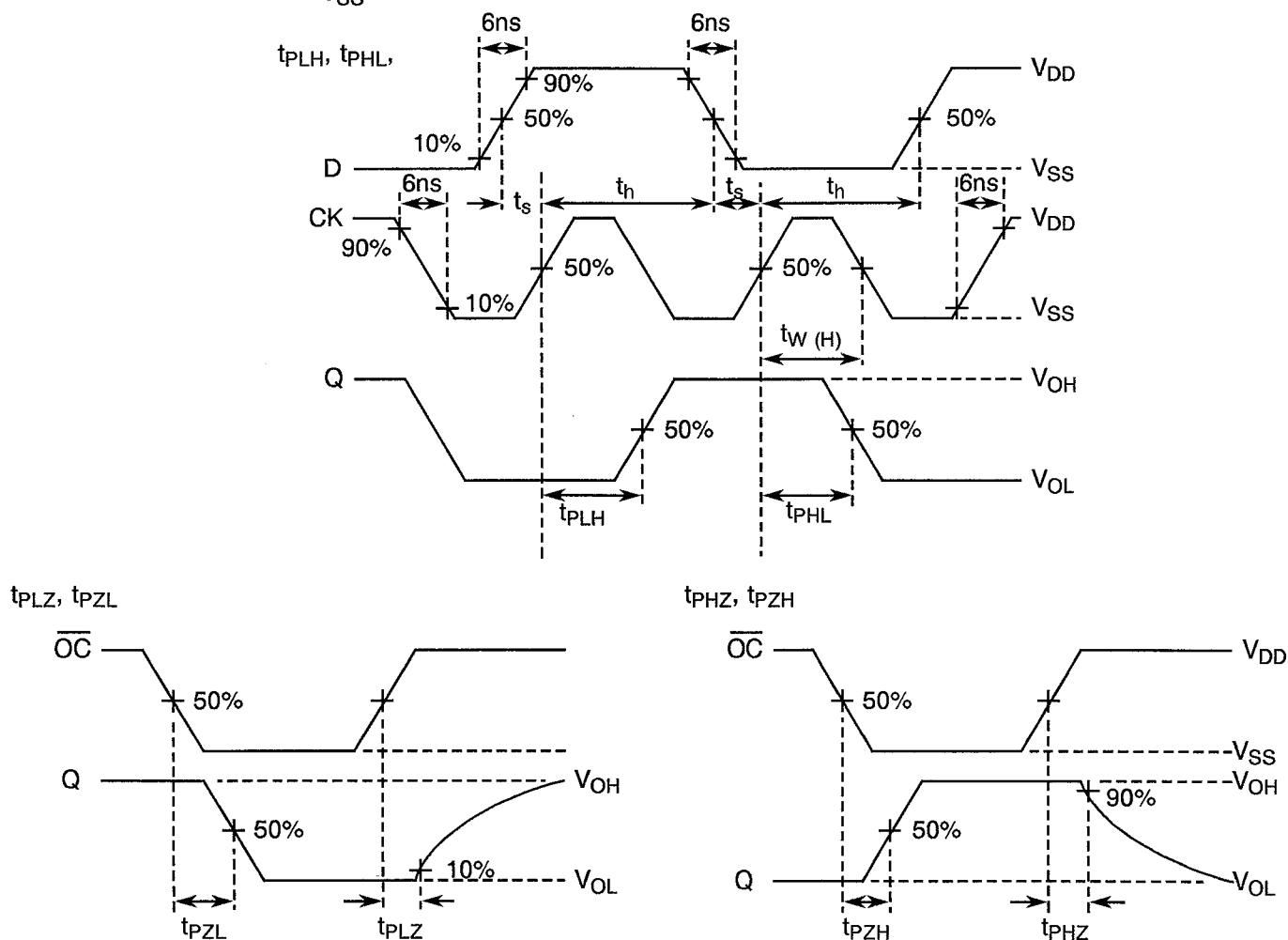
VOLTAGE WAVEFORMS
