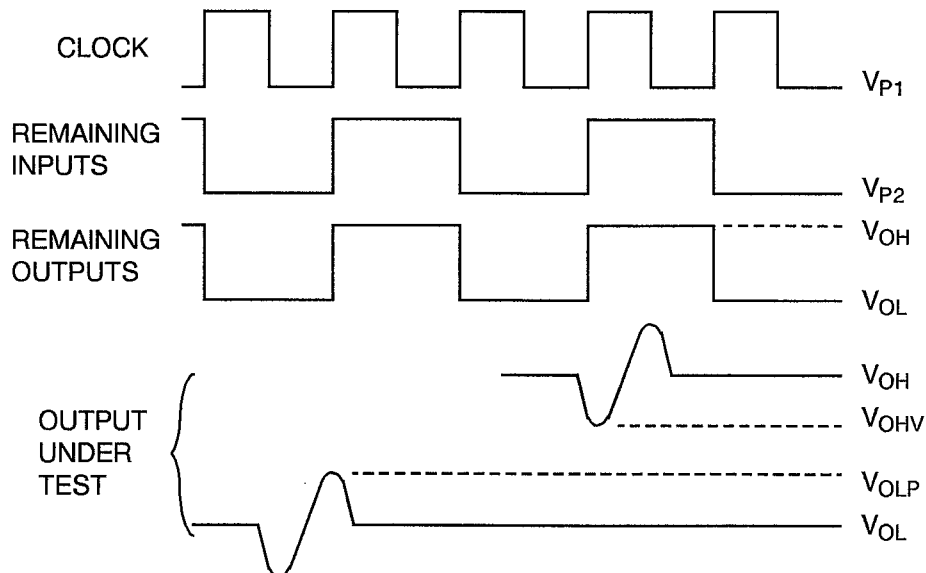
SIGNAL WAVEFORMS
