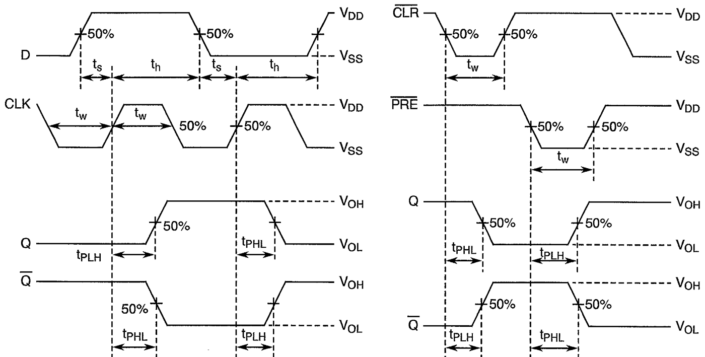
VOLTAGE WAVEFORMS
