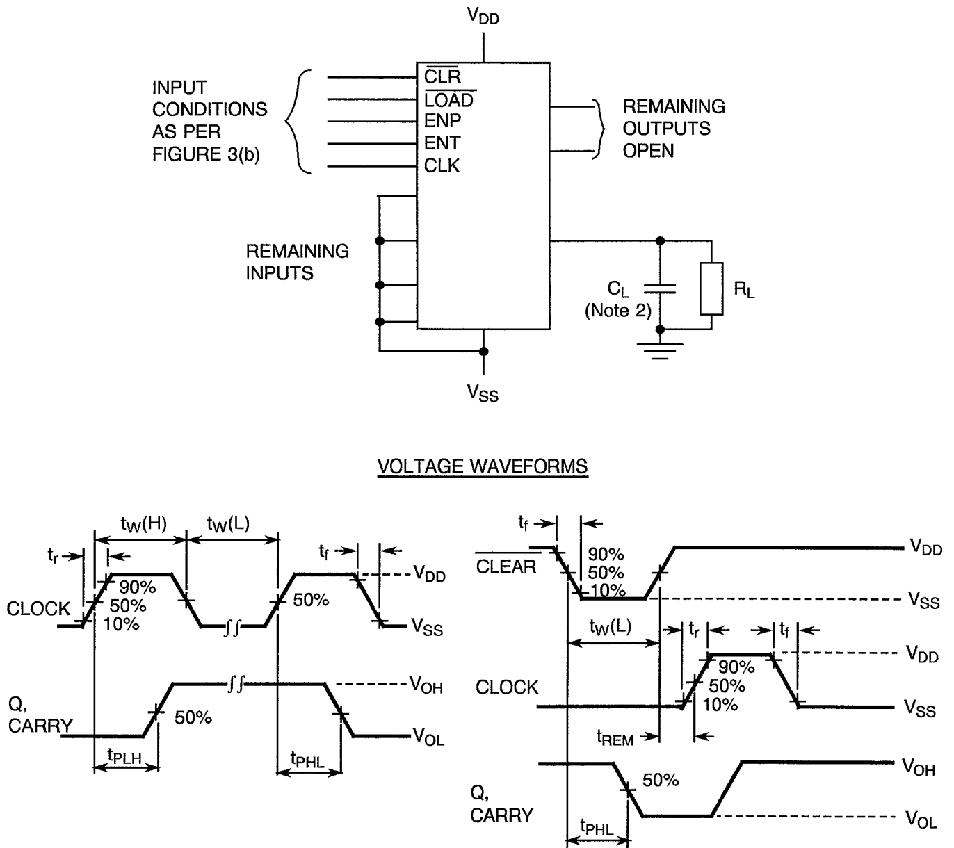
FIGURE 4(h) - PROPAGATION DELAY
