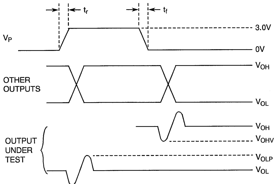
VOLTAGE WAVEFORMS
