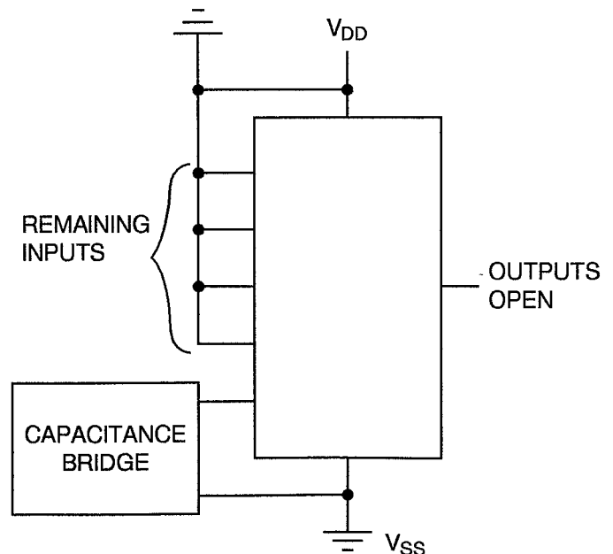
FIGURE 4(i) - INPUT CAPACITANCE
