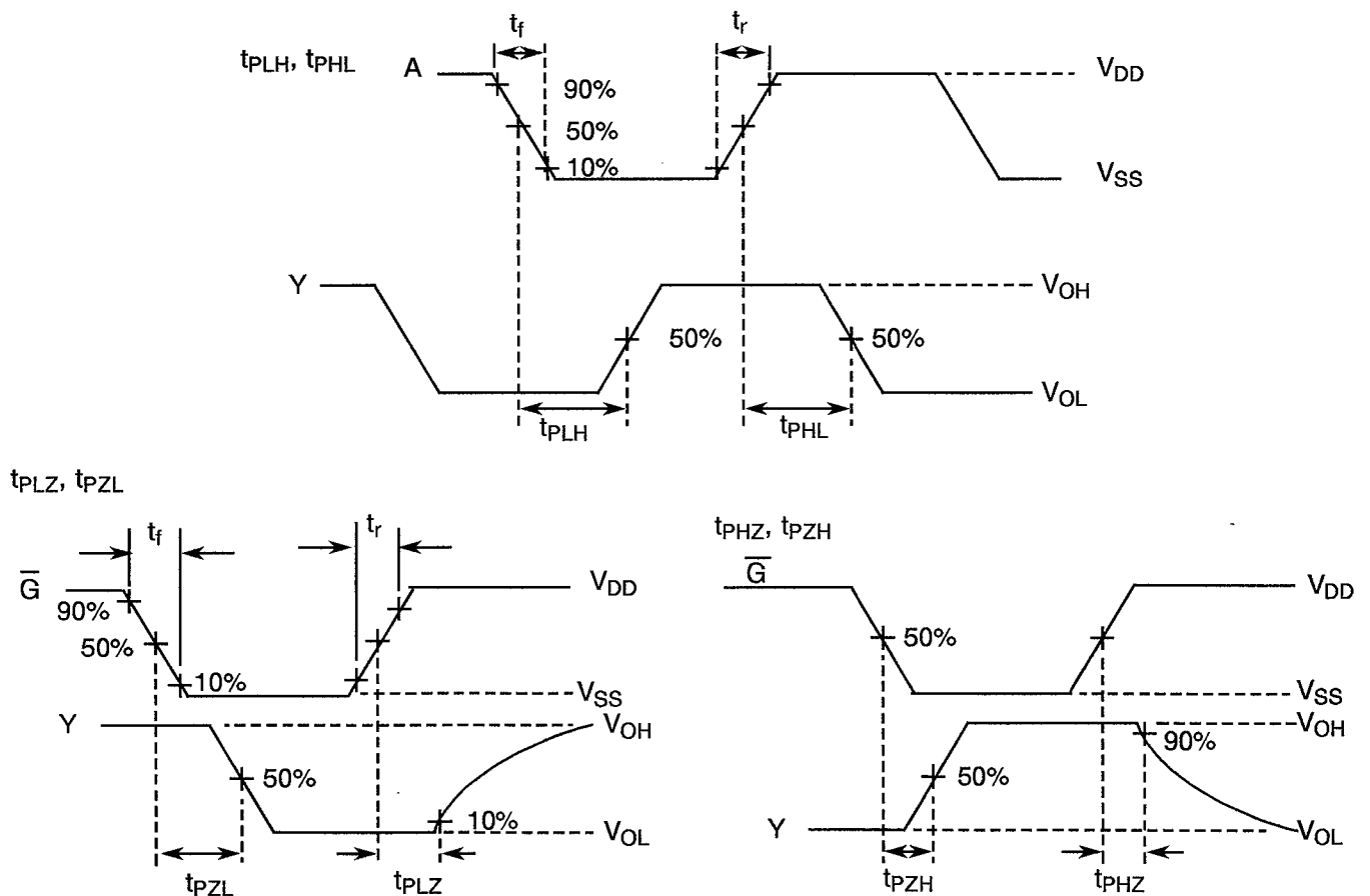
VOLTAGE WAVEFORMS
