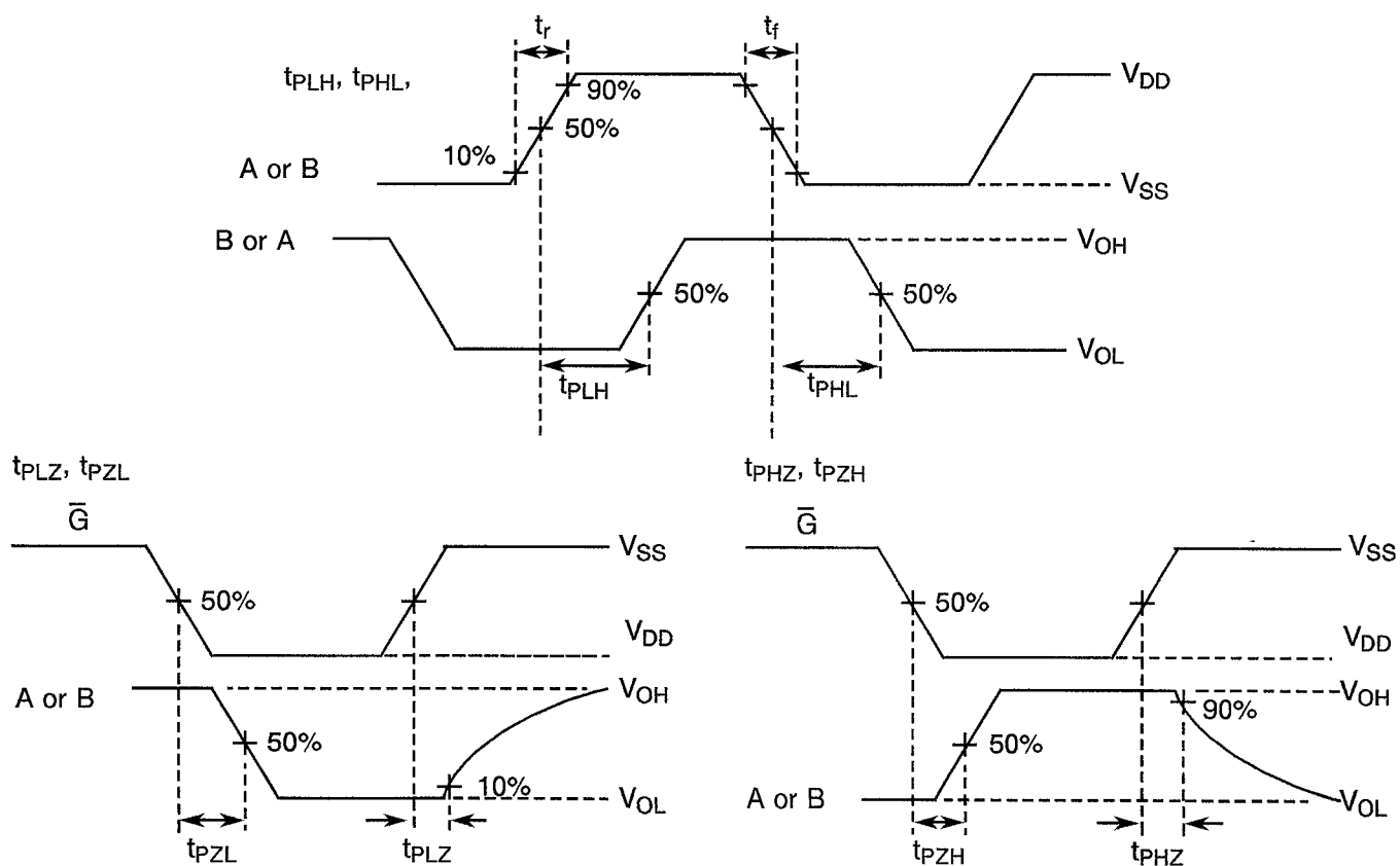
VOLTAGE WAVEFORMS
