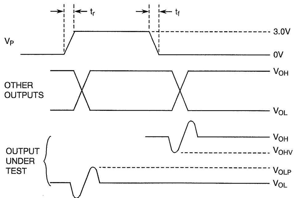
VOLTAGE WAVEFORMS
